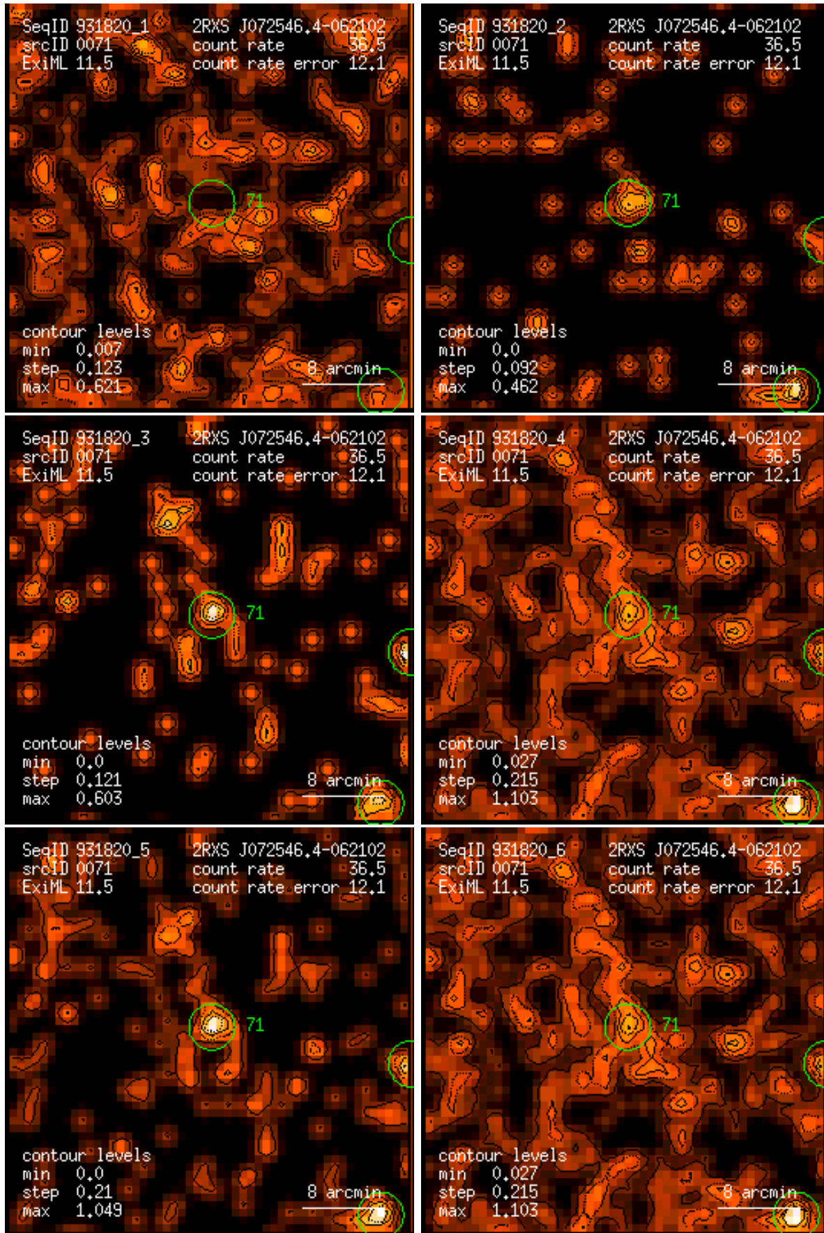
Figure 71: RASS 931820: detection 0071: band rate images, Gaussian filter: (1) PSPC channels 11 – 41, (2) 52 – 90, (3) 91 – 201, (4) 11 – 235, (5) 52 – 201, (6) 11 – 201. Broad band rates in counts/ks. Band rate contour levels in counts/ks/arcmin 2 .
