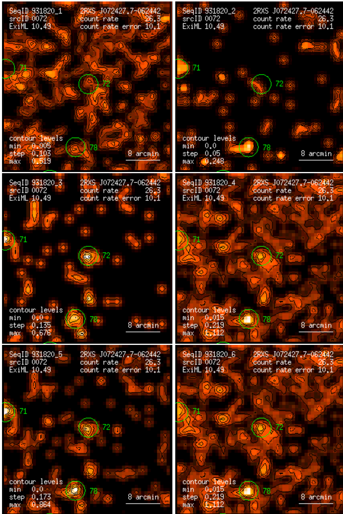
Figure 72: RASS 931820: detection 0072: band rate images, Gaussian filter: (1) PSPC channels 11 – 41, (2) 52 – 90, (3) 91 – 201, (4) 11 – 235, (5) 52 – 201, (6) 11 – 201. Broad band rates in counts/ks. Band rate contour levels in counts/ks/arcmin 2 .
