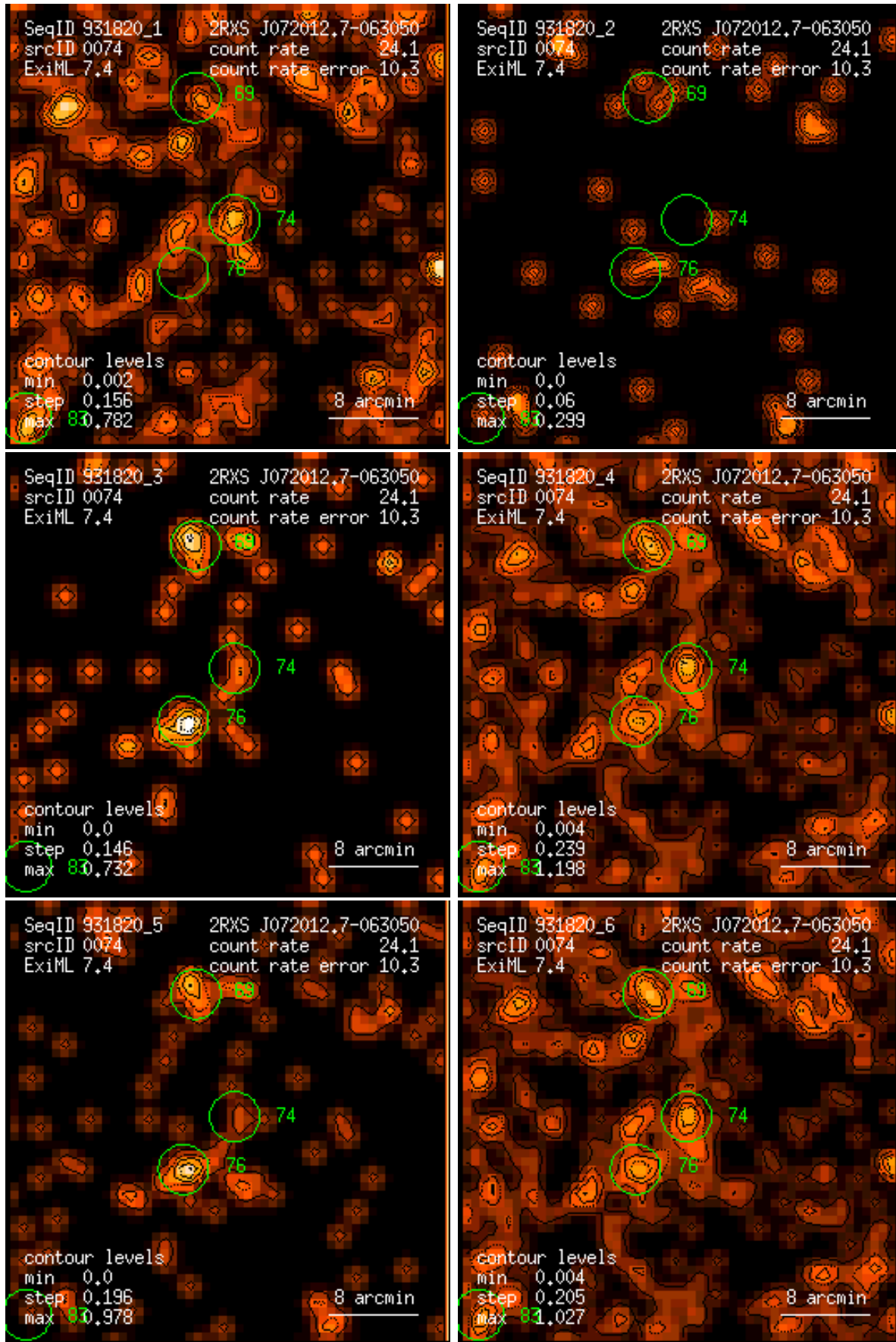
Figure 74: RASS 931820: detection 0074: band rate images, Gaussian filter: (1) PSPC channels 11 – 41, (2) 52 – 90, (3) 91 – 201, (4) 11 – 235, (5) 52 – 201, (6) 11 – 201. Broad band rates in counts/ks. Band rate contour levels in counts/ks/arcmin 2 .
