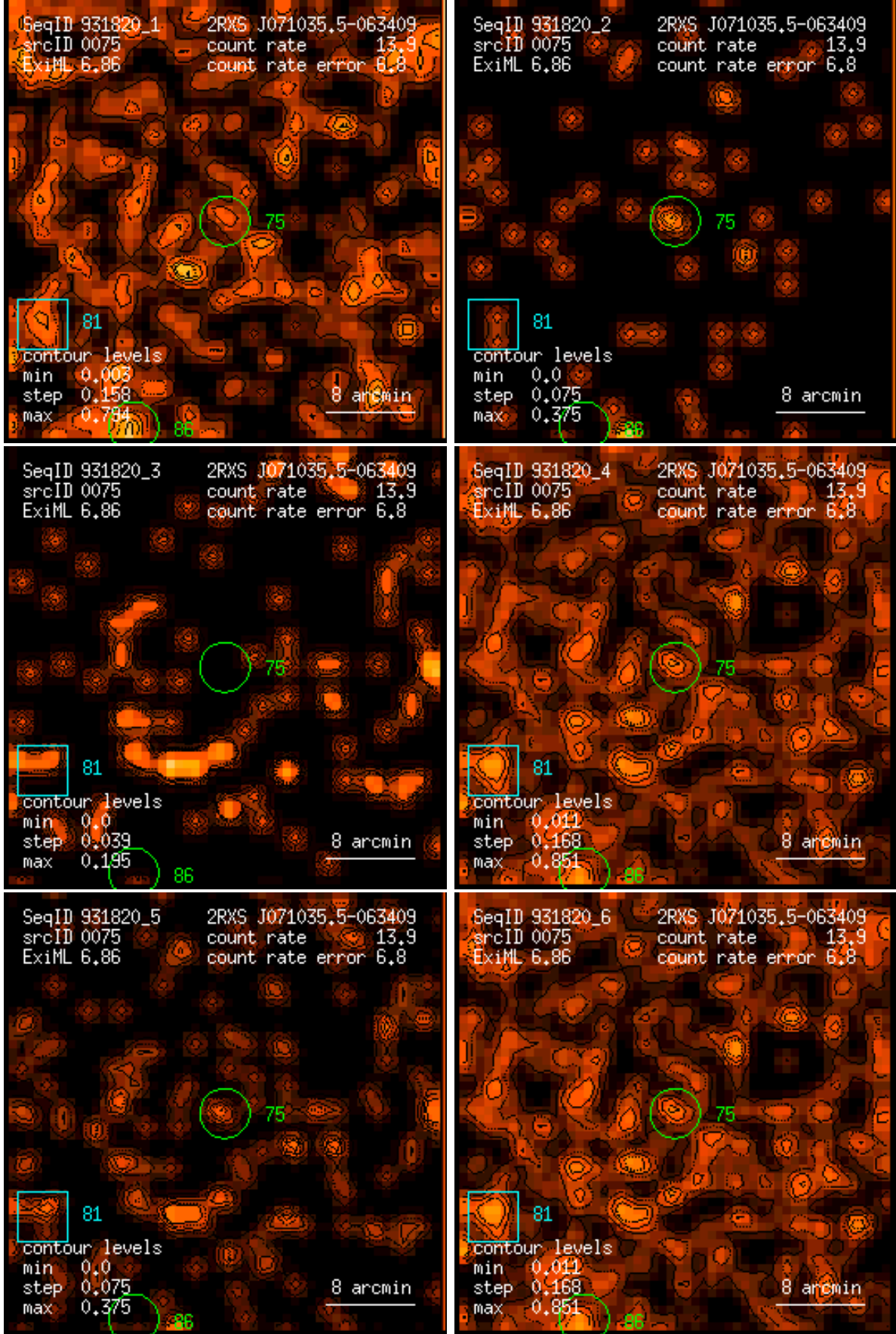
Figure 75: RASS 931820: detection 0075: band rate images, Gaussian filter: (1) PSPC channels 11 – 41, (2) 52 – 90, (3) 91 – 201, (4) 11 – 235, (5) 52 – 201, (6) 11 – 201. Broad band rates in counts/ks. Band rate contour levels in counts/ks/arcmin 2 .
