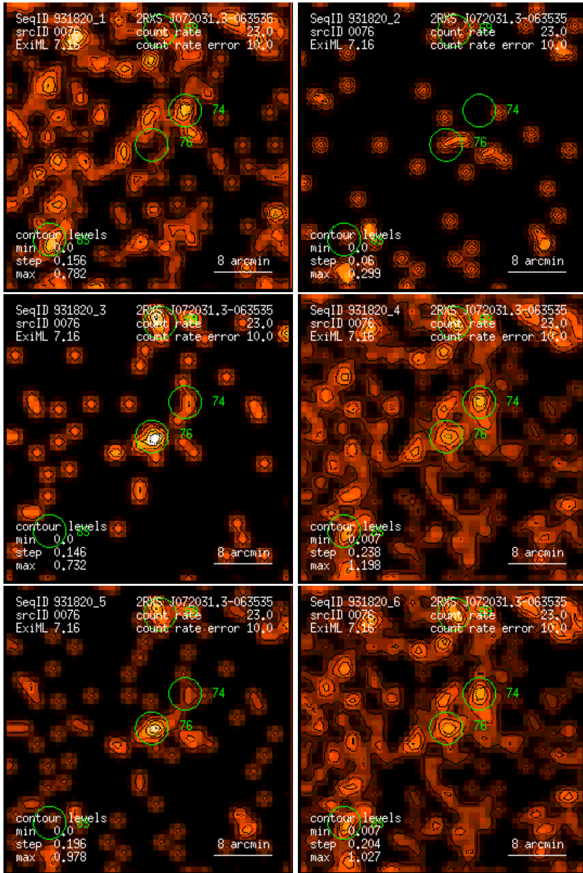
Figure 76: RASS 931820: detection 0076: band rate images, Gaussian filter: (1) PSPC channels 11 – 41, (2) 52 – 90, (3) 91 – 201, (4) 11 – 235, (5) 52 – 201, (6) 11 – 201. Broad band rates in counts/ks. Band rate contour levels in counts/ks/arcmin 2 .
