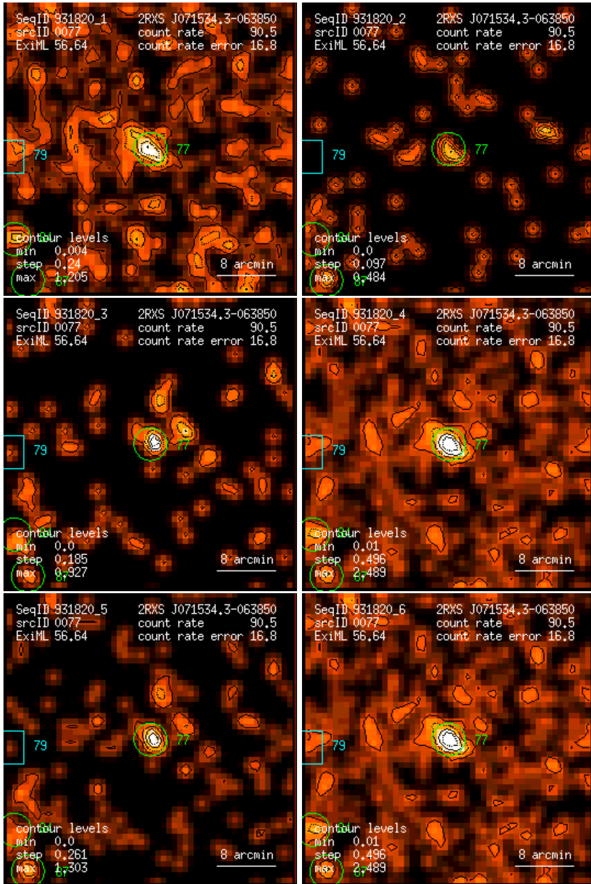
Figure 77: RASS 931820: detection 0077: band rate images, Gaussian filter: (1) PSPC channels 11 – 41, (2) 52 – 90, (3) 91 – 201, (4) 11 – 235, (5) 52 – 201, (6) 11 – 201. Broad band rates in counts/ks. Band rate contour levels in counts/ks/arcmin 2 .
