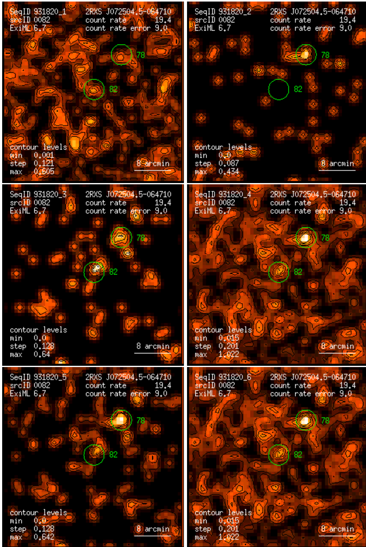
Figure 82: RASS 931820: detection 0082: band rate images, Gaussian filter: (1) PSPC channels 11 – 41, (2) 52 – 90, (3) 91 – 201, (4) 11 – 235, (5) 52 – 201, (6) 11 – 201. Broad band rates in counts/ks. Band rate contour levels in counts/ks/arcmin 2 .
