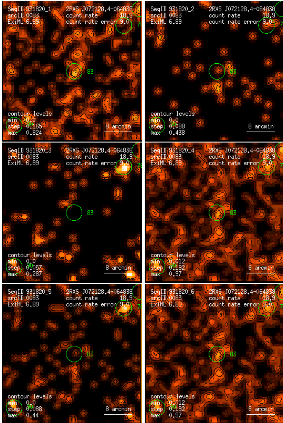
Figure 83: RASS 931820: detection 0083: band rate images, Gaussian filter: (1) PSPC channels 11 – 41, (2) 52 – 90, (3) 91 – 201, (4) 11 – 235, (5) 52 – 201, (6) 11 – 201. Broad band rates in counts/ks. Band rate contour levels in counts/ks/arcmin 2 .
