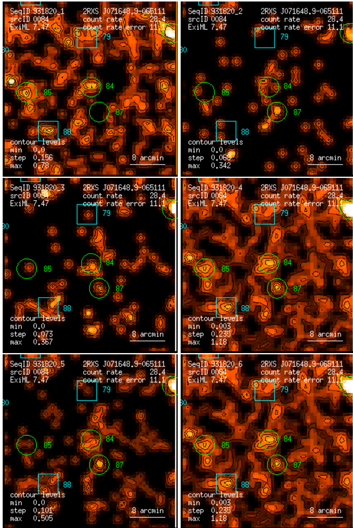
Figure 84: RASS 931820: detection 0084: band rate images, Gaussian filter: (1) PSPC channels 11 – 41, (2) 52 – 90, (3) 91 – 201, (4) 11 – 235, (5) 52 – 201, (6) 11 – 201. Broad band rates in counts/ks. Band rate contour levels in counts/ks/arcmin 2 .
