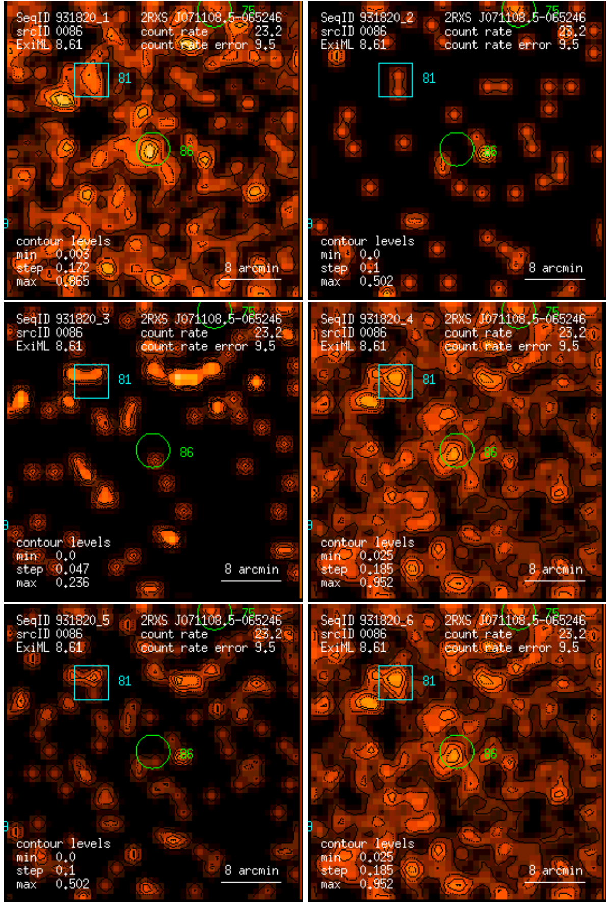
Figure 86: RASS 931820: detection 0086: band rate images, Gaussian filter: (1) PSPC channels 11 – 41, (2) 52 – 90, (3) 91 – 201, (4) 11 – 235, (5) 52 – 201, (6) 11 – 201. Broad band rates in counts/ks. Band rate contour levels in counts/ks/arcmin 2 .
