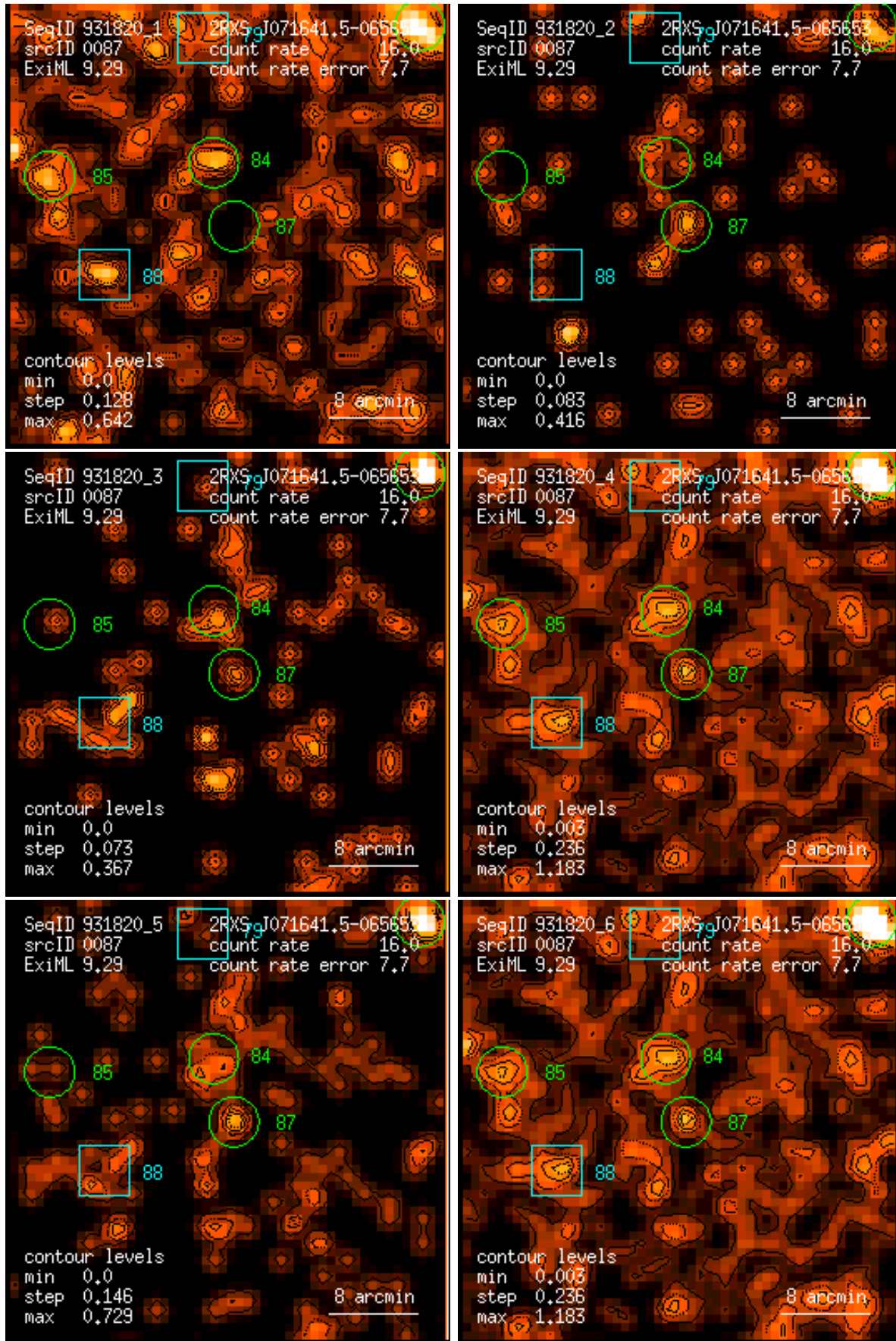
Figure 87: RASS 931820: detection 0087: band rate images, Gaussian filter: (1) PSPC channels 11 – 41, (2) 52 – 90, (3) 91 – 201, (4) 11 – 235, (5) 52 – 201, (6) 11 – 201. Broad band rates in counts/ks. Band rate contour levels in counts/ks/arcmin 2 .
