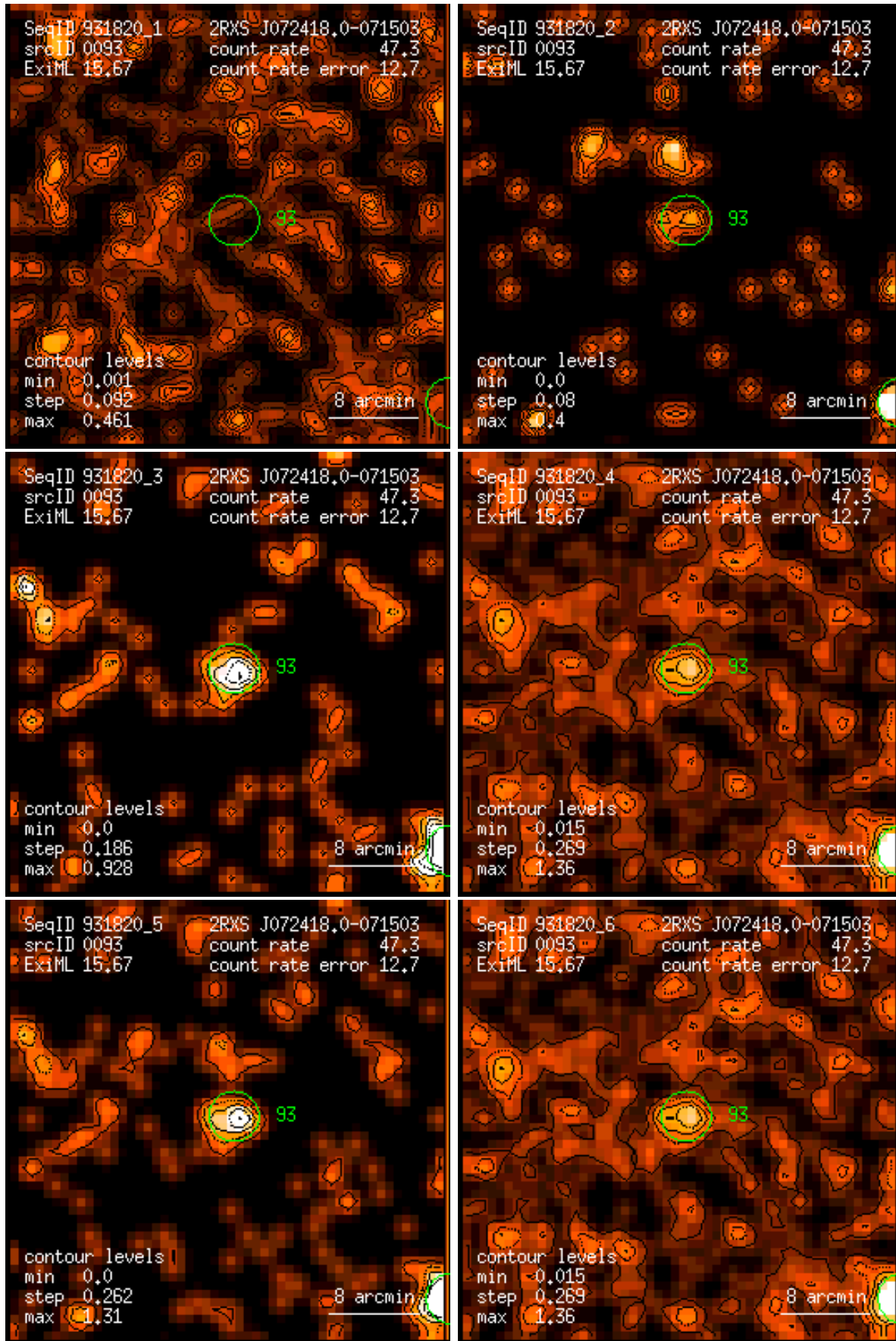
Figure 93: RASS 931820: detection 0093: band rate images, Gaussian filter: (1) PSPC channels 11 – 41, (2) 52 – 90, (3) 91 – 201, (4) 11 – 235, (5) 52 – 201, (6) 11 – 201. Broad band rates in counts/ks. Band rate contour levels in counts/ks/arcmin 2 .
