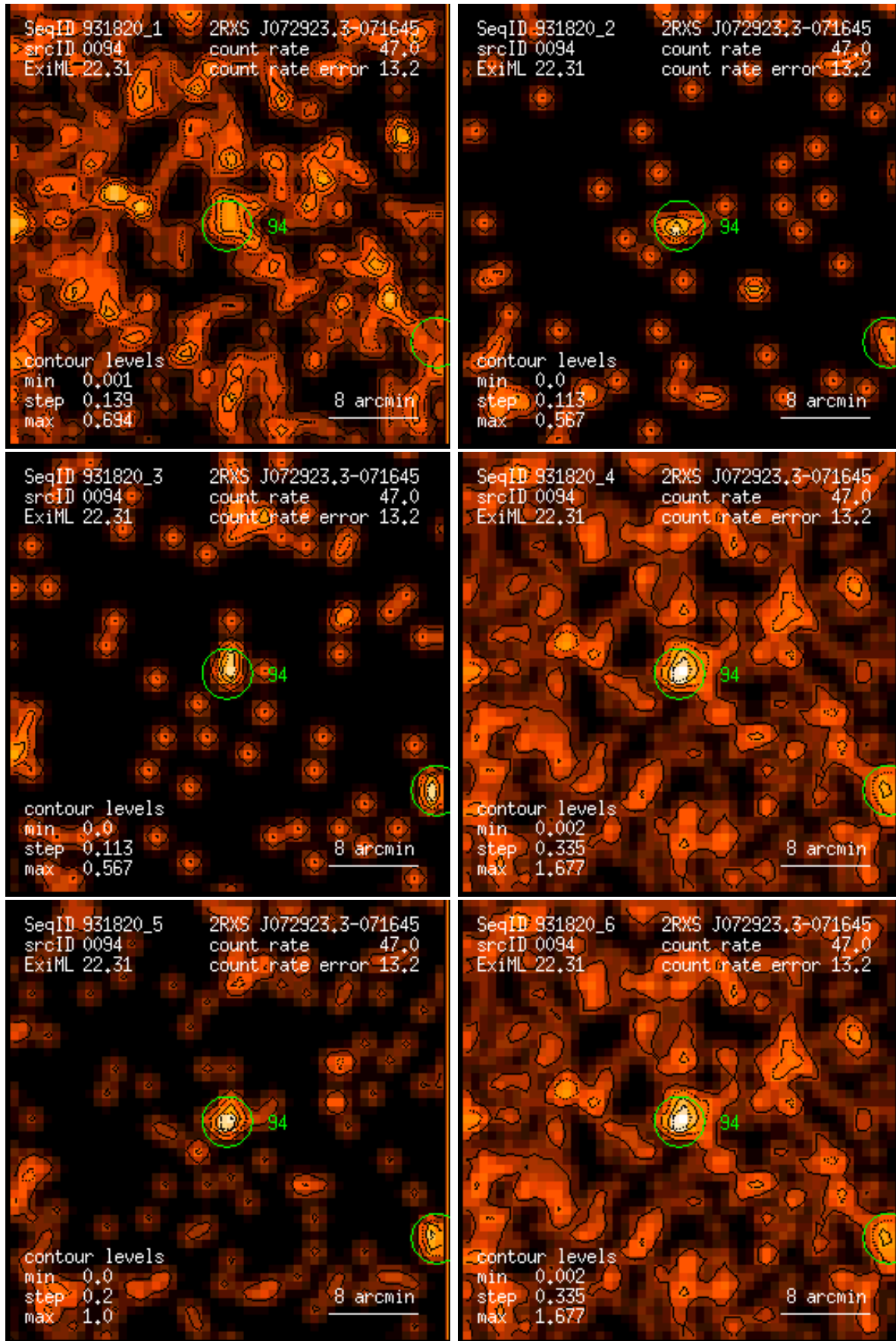
Figure 94: RASS 931820: detection 0094: band rate images, Gaussian filter: (1) PSPC channels 11 – 41, (2) 52 – 90, (3) 91 – 201, (4) 11 – 235, (5) 52 – 201, (6) 11 – 201. Broad band rates in counts/ks. Band rate contour levels in counts/ks/arcmin 2 .
