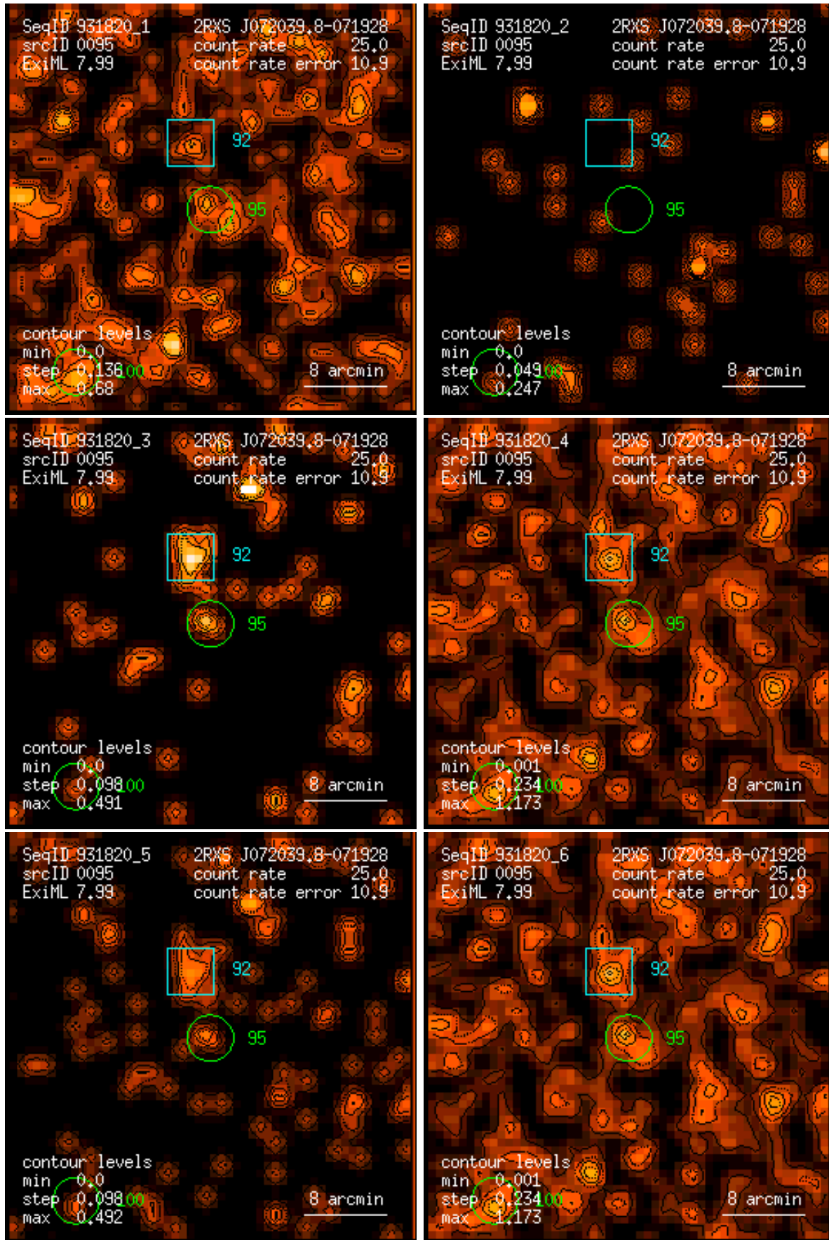
Figure 95: RASS 931820: detection 0095: band rate images, Gaussian filter: (1) PSPC channels 11 – 41, (2) 52 – 90, (3) 91 – 201, (4) 11 – 235, (5) 52 – 201, (6) 11 – 201. Broad band rates in counts/ks. Band rate contour levels in counts/ks/arcmin 2 .
