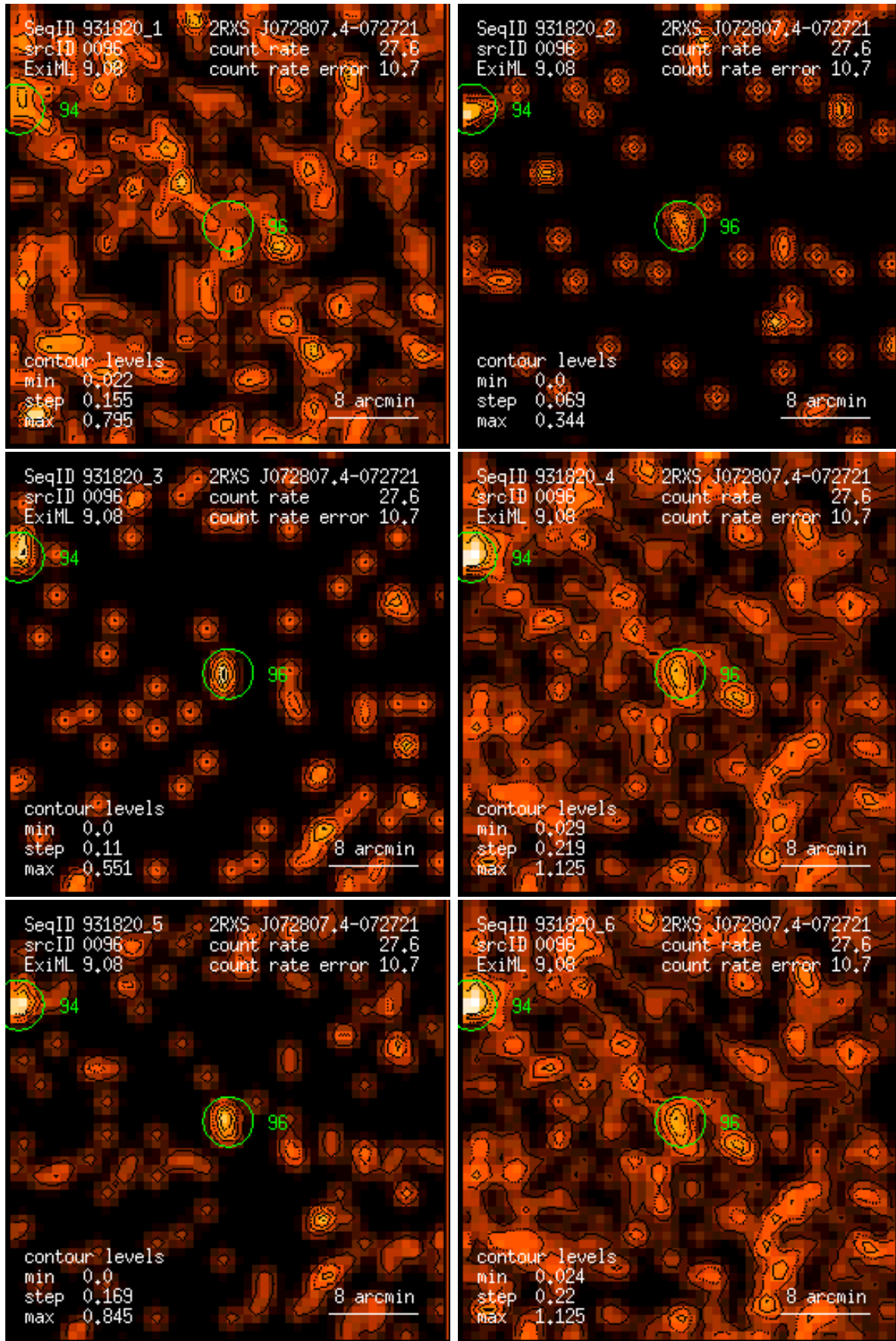
Figure 96: RASS 931820: detection 0096: band rate images, Gaussian filter: (1) PSPC channels 11 – 41, (2) 52 – 90, (3) 91 – 201, (4) 11 – 235, (5) 52 – 201, (6) 11 – 201. Broad band rates in counts/ks. Band rate contour levels in counts/ks/arcmin 2 .
