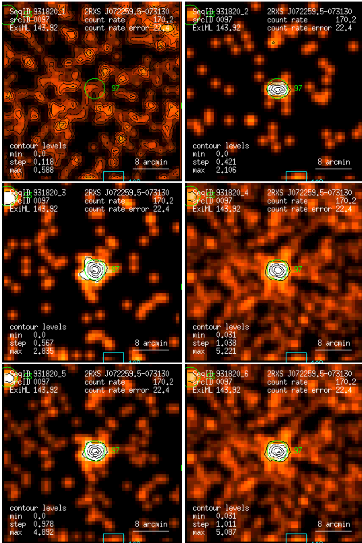
Figure 97: RASS 931820: detection 0097: band rate images, Gaussian filter: (1) PSPC channels 11 – 41, (2) 52 – 90, (3) 91 – 201, (4) 11 – 235, (5) 52 – 201, (6) 11 – 201. Broad band rates in counts/ks. Band rate contour levels in counts/ks/arcmin 2 .
