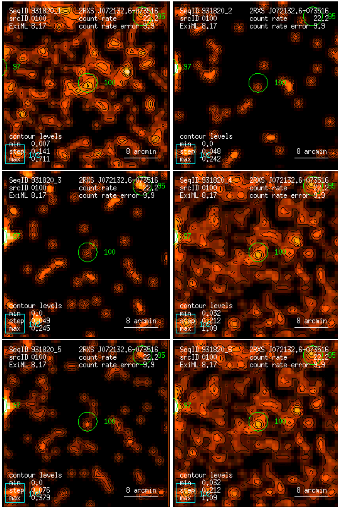
Figure 100: RASS 931820: detection 0100: band rate images, Gaussian filter: (1) PSPC channels 11 – 41, (2) 52 – 90, (3) 91 – 201, (4) 11 – 235, (5) 52 – 201, (6) 11 – 201. Broad band rates in counts/ks. Band rate contour levels in counts/ks/arcmin 2 .
