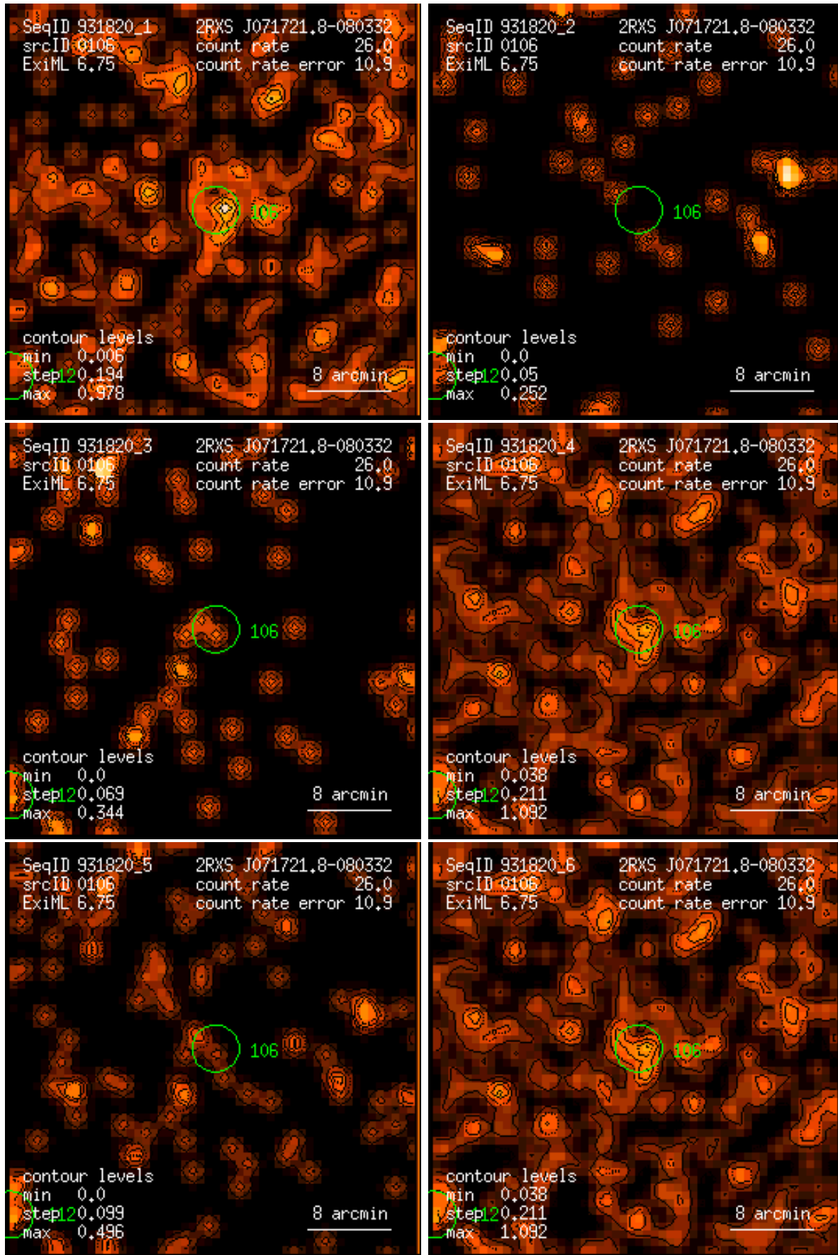
Figure 106: RASS 931820: detection 0106: band rate images, Gaussian filter: (1) PSPC channels 11 – 41, (2) 52 – 90, (3) 91 – 201, (4) 11 – 235, (5) 52 – 201, (6) 11 – 201. Broad band rates in counts/ks. Band rate contour levels in counts/ks/arcmin 2 .
