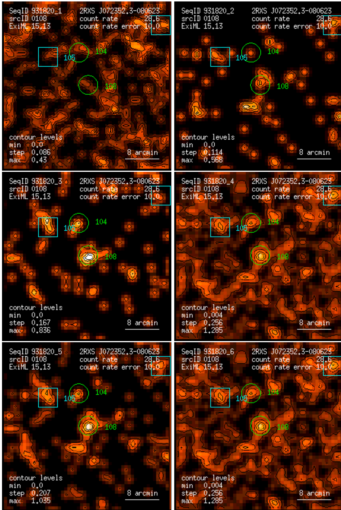
Figure 108: RASS 931820: detection 0108: band rate images, Gaussian filter: (1) PSPC channels 11 – 41, (2) 52 – 90, (3) 91 – 201, (4) 11 – 235, (5) 52 – 201, (6) 11 – 201. Broad band rates in counts/ks. Band rate contour levels in counts/ks/arcmin 2 .
