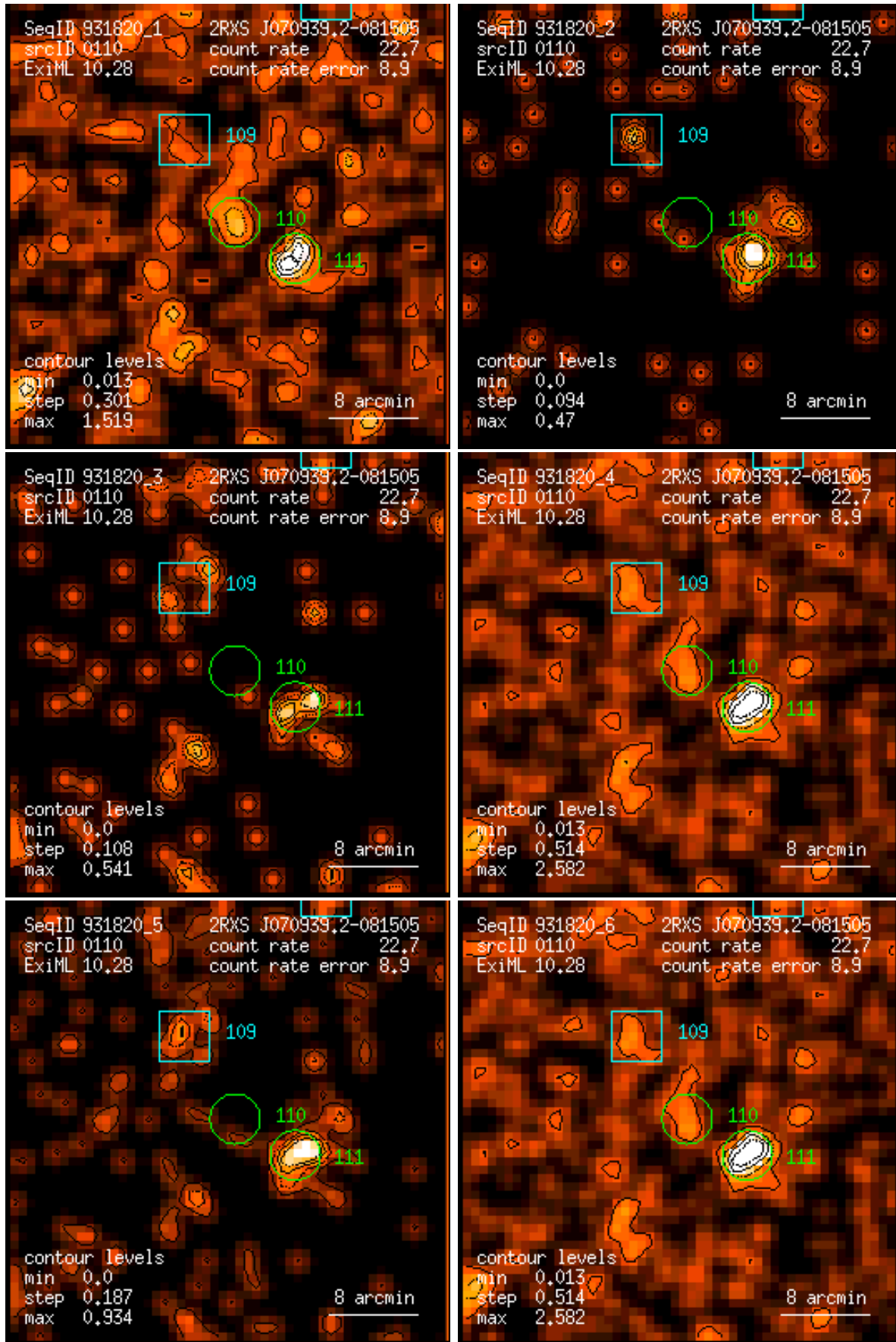
Figure 110: RASS 931820: detection 0110: band rate images, Gaussian filter: (1) PSPC channels 11 – 41, (2) 52 – 90, (3) 91 – 201, (4) 11 – 235, (5) 52 – 201, (6) 11 – 201. Broad band rates in counts/ks. Band rate contour levels in counts/ks/arcmin 2 .
