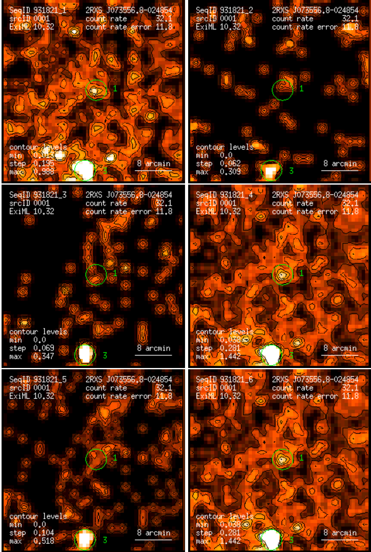
Figure 1: RASS 931821: detection 0001: band rate images, Gaussian filter: (1) PSPC channels 11 – 41, (2) 52 – 90, (3) 91 – 201, (4) 11 – 235, (5) 52 – 201, (6) 11 – 201. Broad band rates in counts/ks. Band rate contour levels in counts/ks/arcmin 2 .
