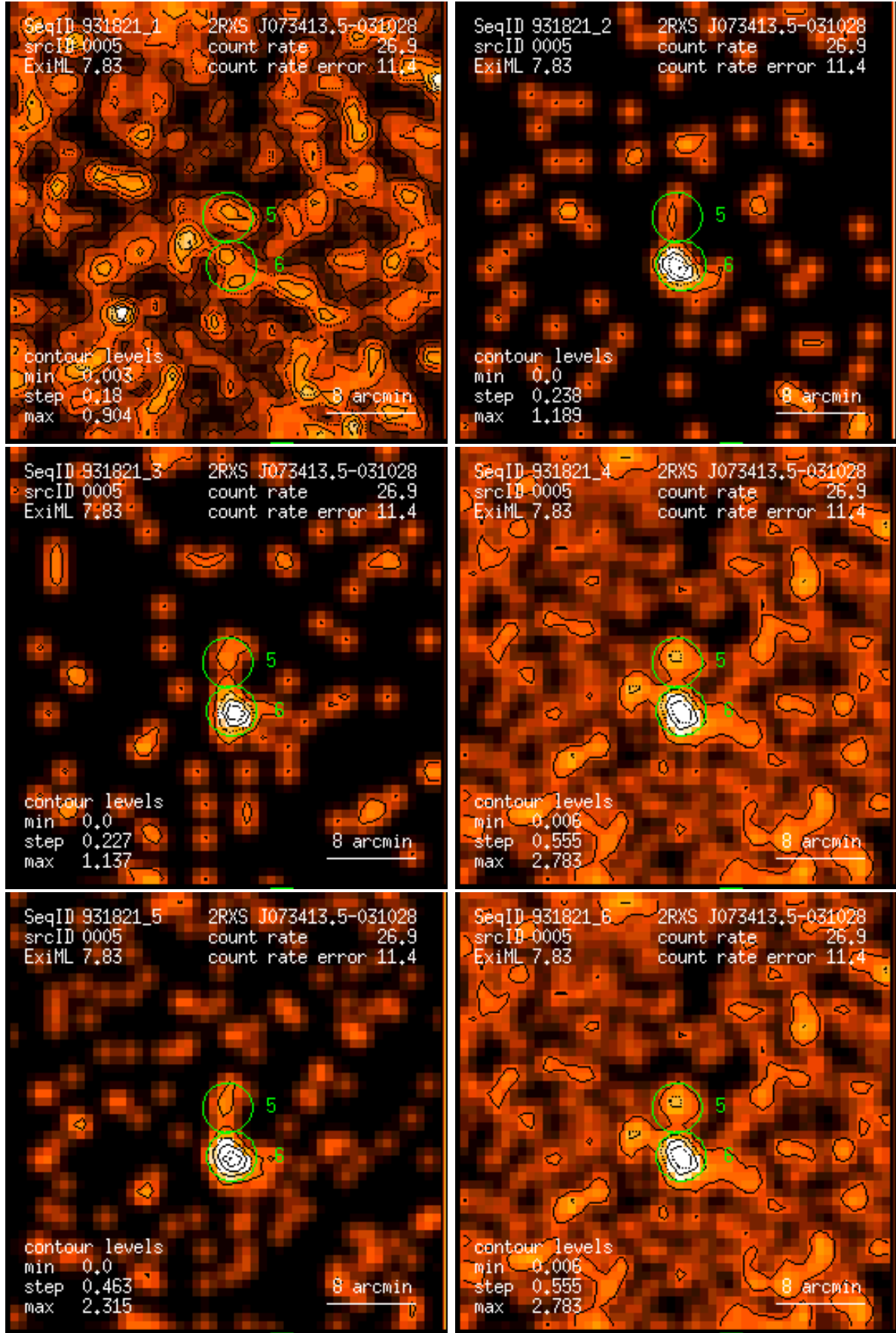
Figure 5: RASS 931821: detection 0005: band rate images, Gaussian filter: (1) PSPC channels 11 – 41, (2) 52 – 90, (3) 91 – 201, (4) 11 – 235, (5) 52 – 201, (6) 11 – 201. Broad band rates in counts/ks. Band rate contour levels in counts/ks/arcmin 2 .
