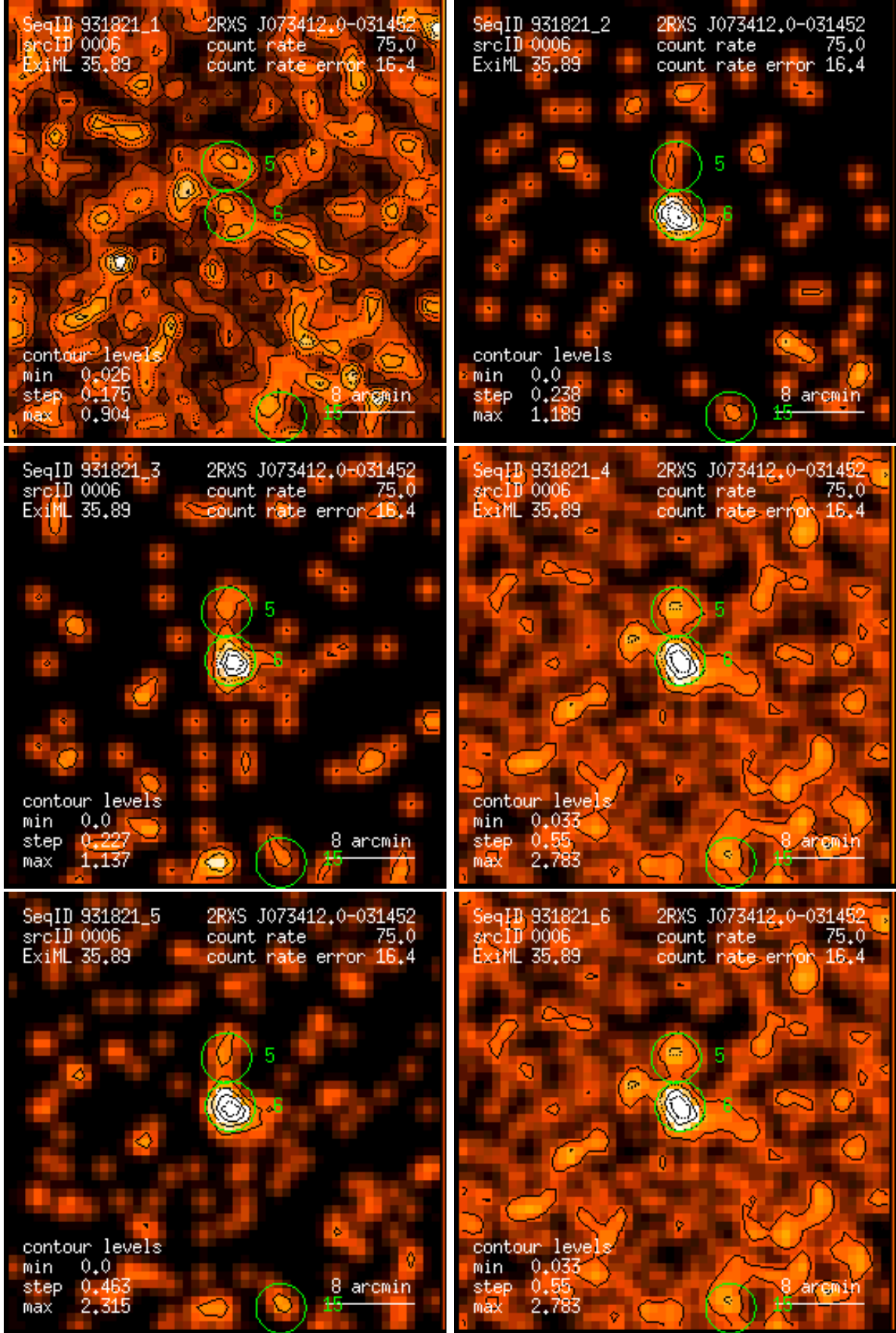
Figure 6: RASS 931821: detection 0006: band rate images, Gaussian filter: (1) PSPC channels 11 – 41, (2) 52 – 90, (3) 91 – 201, (4) 11 – 235, (5) 52 – 201, (6) 11 – 201. Broad band rates in counts/ks. Band rate contour levels in counts/ks/arcmin 2 .
