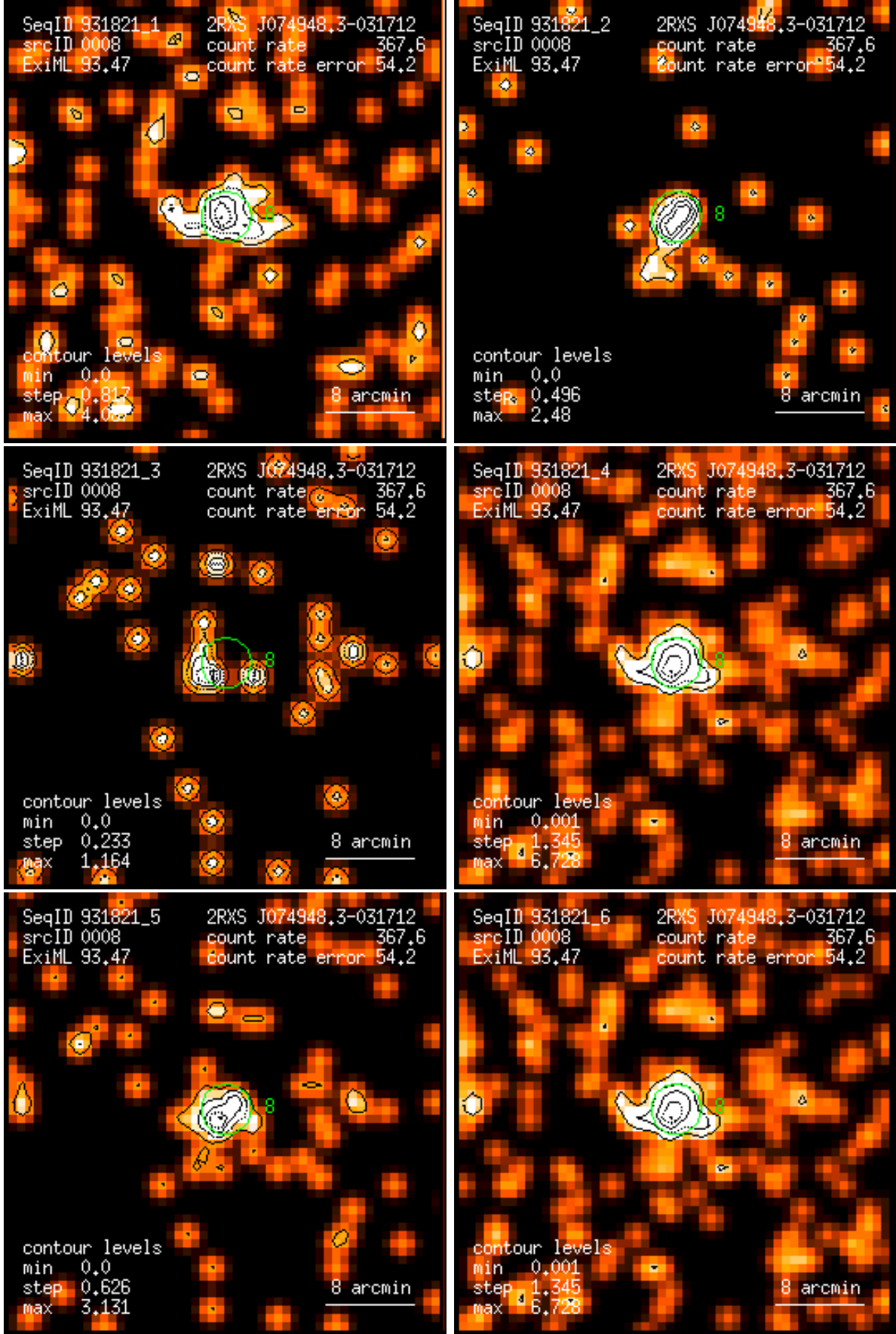
Figure 8: RASS 931821: detection 0008: band rate images, Gaussian filter: (1) PSPC channels 11 – 41, (2) 52 – 90, (3) 91 – 201, (4) 11 – 235, (5) 52 – 201, (6) 11 – 201. Broad band rates in counts/ks. Band rate contour levels in counts/ks/arcmin 2 .
