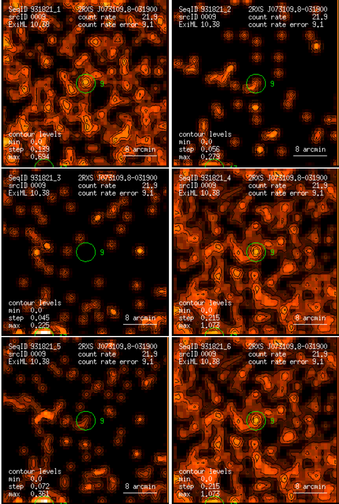
Figure 9: RASS 931821: detection 0009: band rate images, Gaussian filter: (1) PSPC channels 11 – 41, (2) 52 – 90, (3) 91 – 201, (4) 11 – 235, (5) 52 – 201, (6) 11 – 201. Broad band rates in counts/ks. Band rate contour levels in counts/ks/arcmin 2 .
