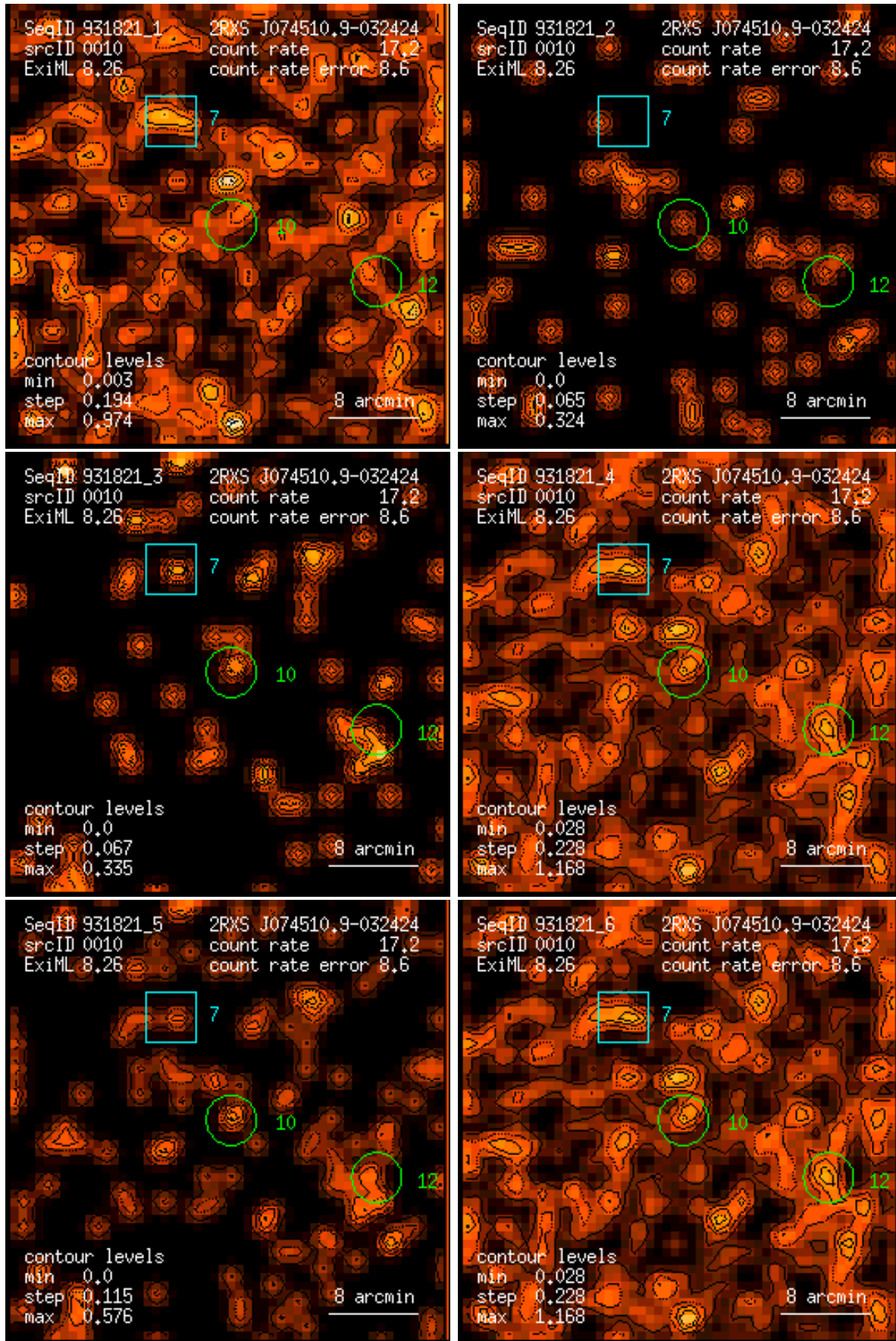
Figure 10: RASS 931821: detection 0010: band rate images, Gaussian filter: (1) PSPC channels 11 – 41, (2) 52 – 90, (3) 91 – 201, (4) 11 – 235, (5) 52 – 201, (6) 11 – 201. Broad band rates in counts/ks. Band rate contour levels in counts/ks/arcmin 2 .
