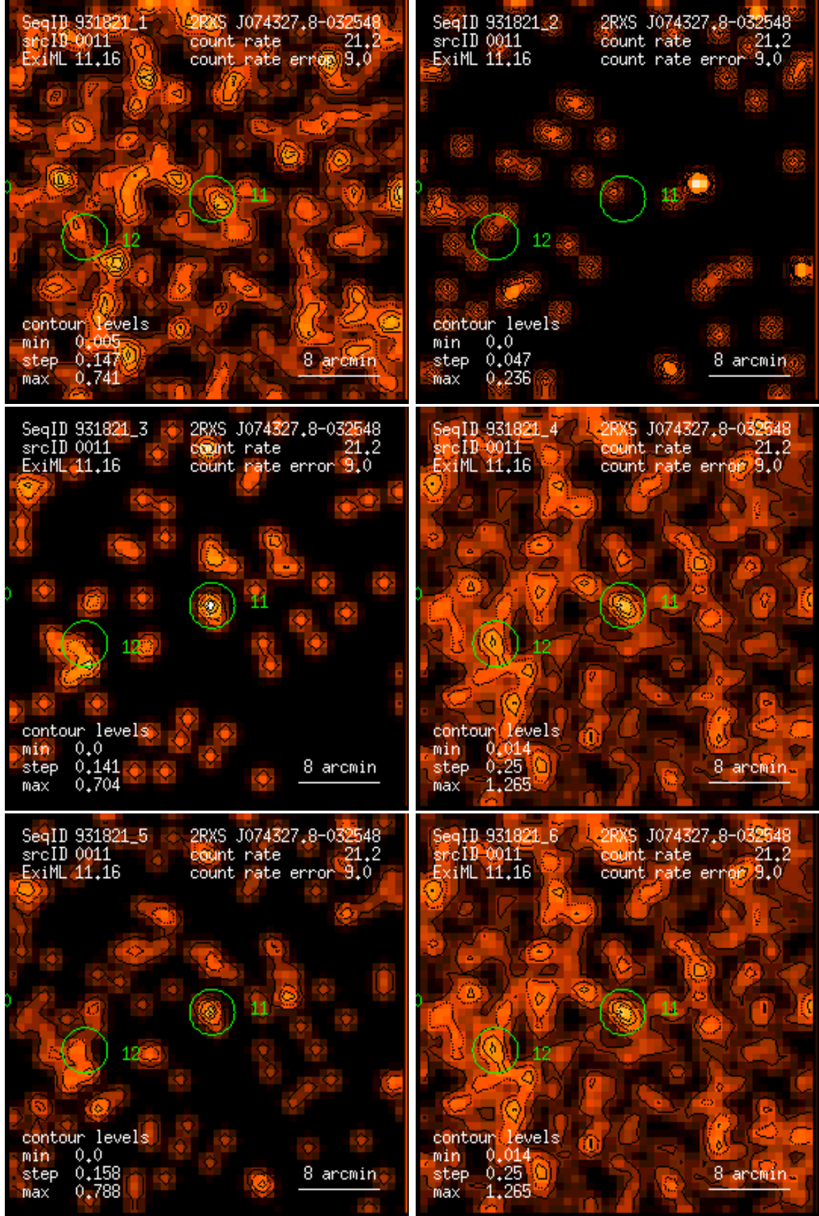
Figure 11: RASS 931821: detection 0011: band rate images, Gaussian filter: (1) PSPC channels 11 – 41, (2) 52 – 90, (3) 91 – 201, (4) 11 – 235, (5) 52 – 201, (6) 11 – 201. Broad band rates in counts/ks. Band rate contour levels in counts/ks/arcmin 2 .
