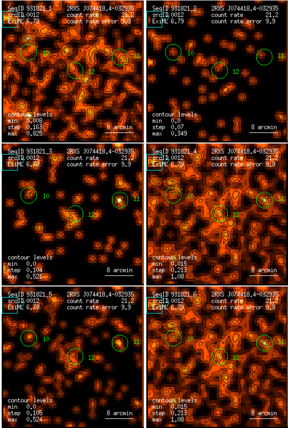
Figure 12: RASS 931821: detection 0012: band rate images, Gaussian filter: (1) PSPC channels 11 – 41, (2) 52 – 90, (3) 91 – 201, (4) 11 – 235, (5) 52 – 201, (6) 11 – 201. Broad band rates in counts/ks. Band rate contour levels in counts/ks/arcmin 2 .
