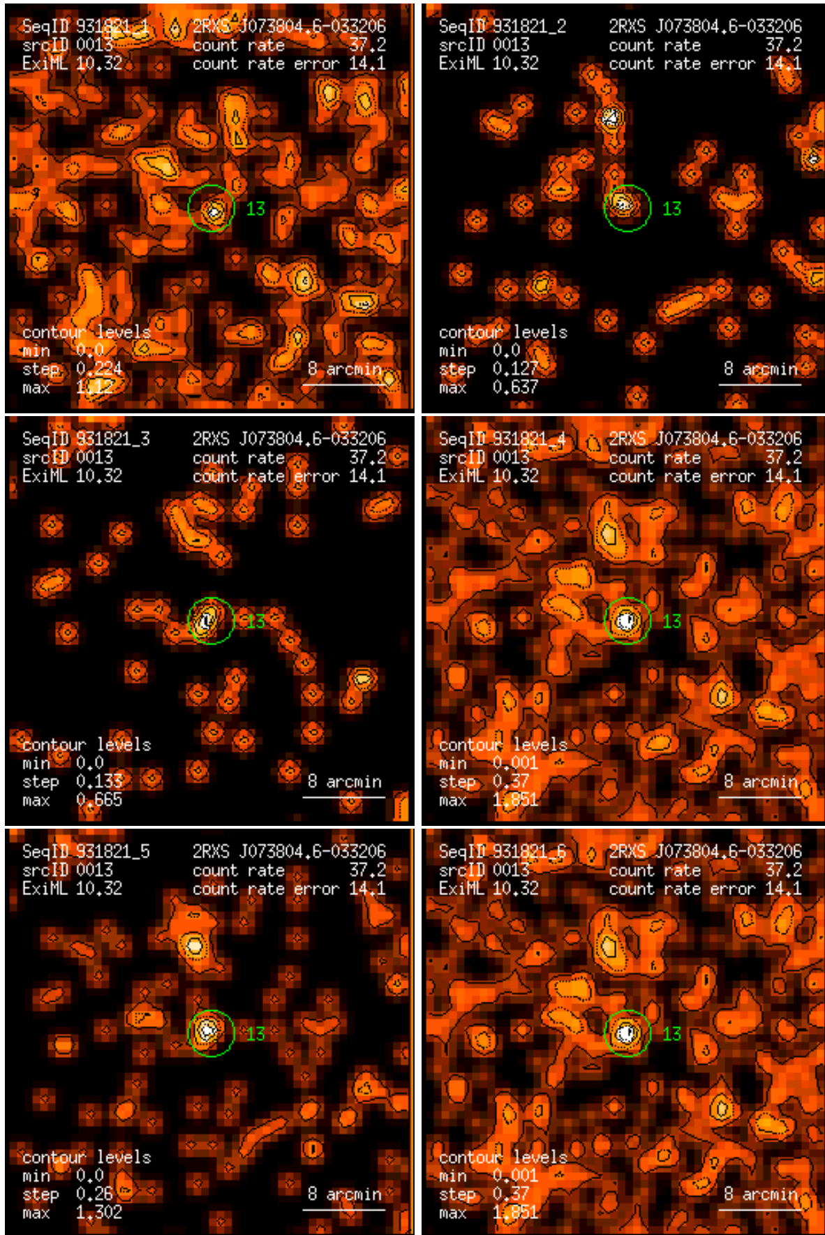
Figure 13: RASS 931821: detection 0013: band rate images, Gaussian filter: (1) PSPC channels 11 – 41, (2) 52 – 90, (3) 91 – 201, (4) 11 – 235, (5) 52 – 201, (6) 11 – 201. Broad band rates in counts/ks. Band rate contour levels in counts/ks/arcmin 2 .
