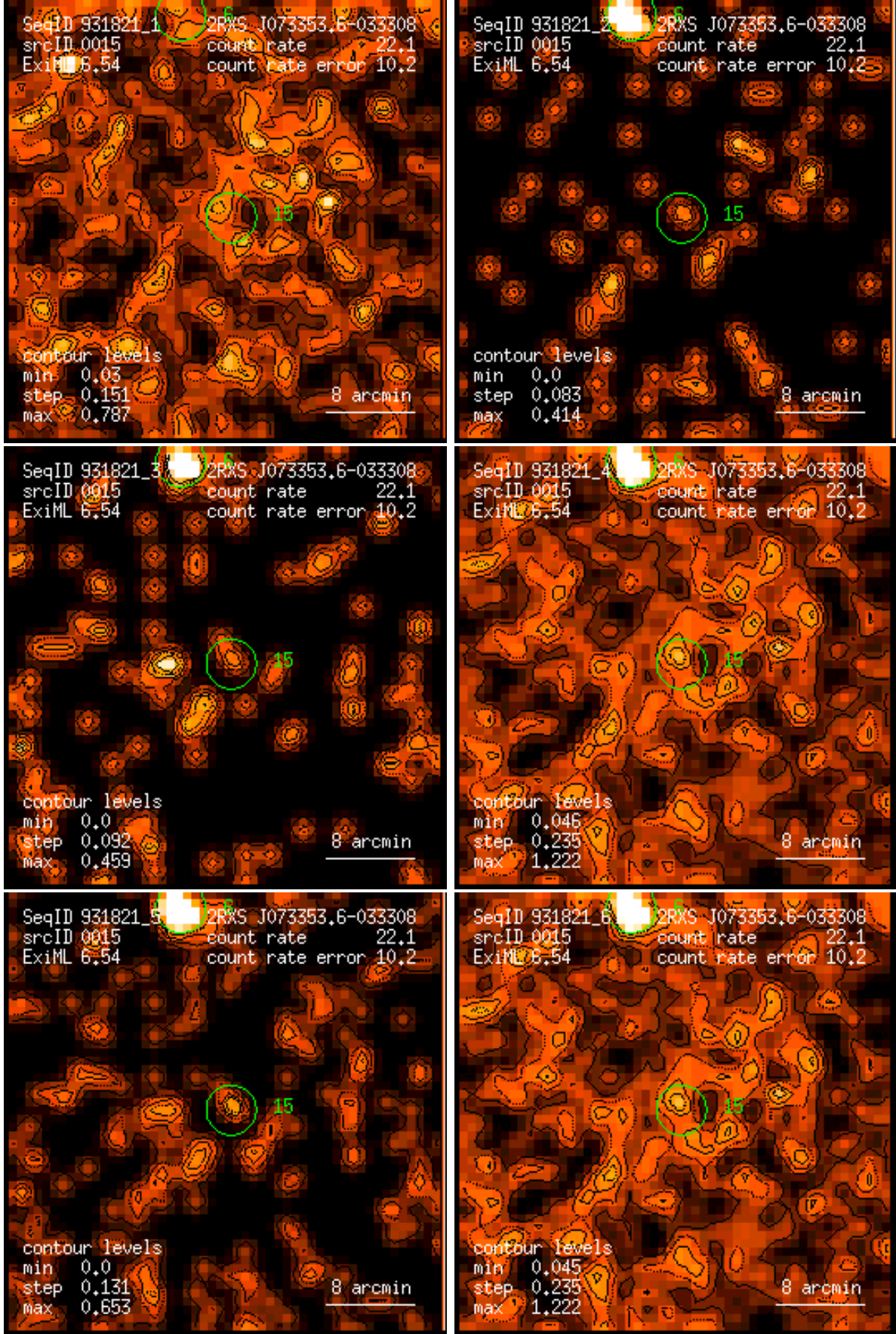
Figure 15: RASS 931821: detection 0015: band rate images, Gaussian filter: (1) PSPC channels 11 – 41, (2) 52 – 90, (3) 91 – 201, (4) 11 – 235, (5) 52 – 201, (6) 11 – 201. Broad band rates in counts/ks. Band rate contour levels in counts/ks/arcmin 2 .
