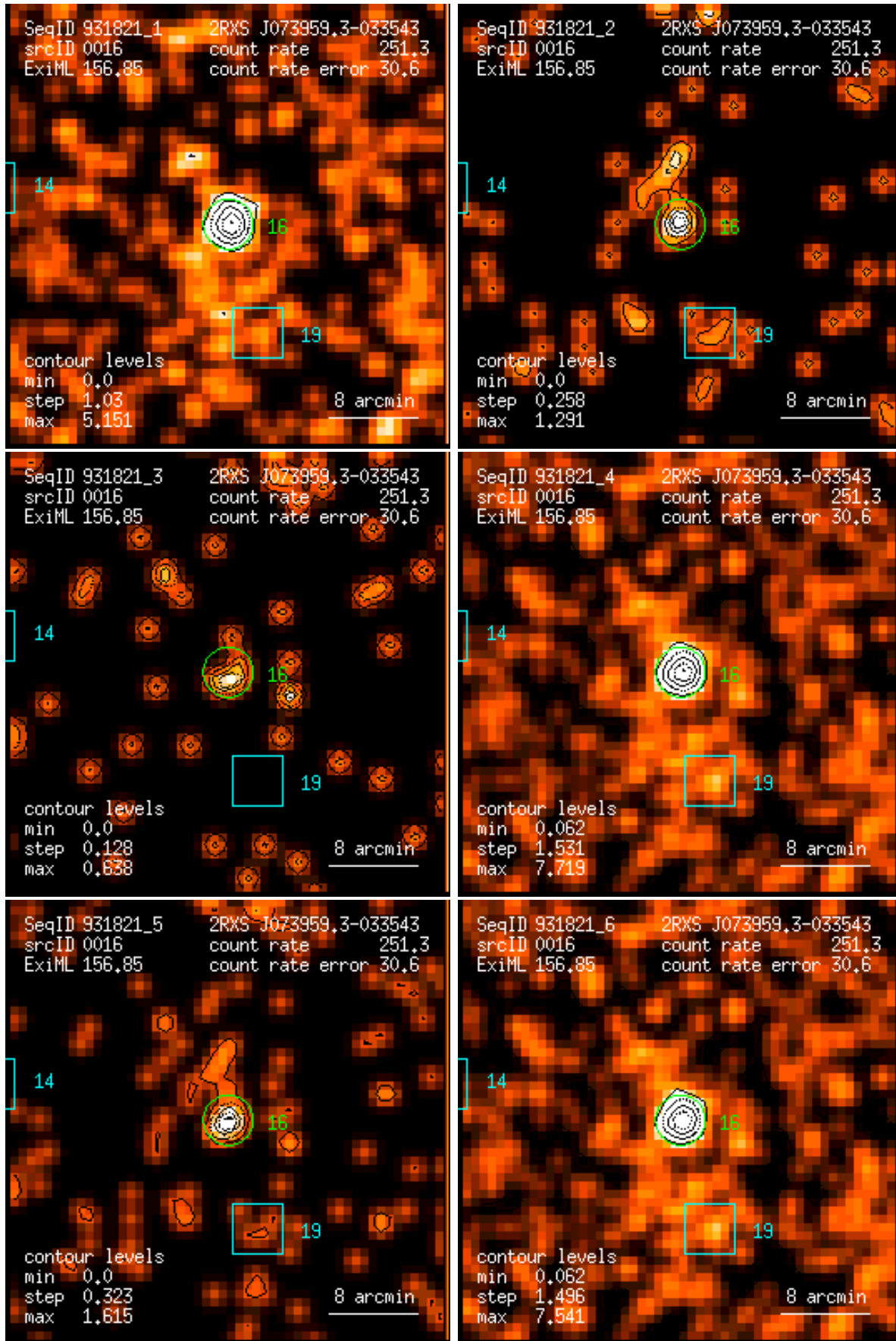
Figure 16: RASS 931821: detection 0016: band rate images, Gaussian filter: (1) PSPC channels 11 – 41, (2) 52 – 90, (3) 91 – 201, (4) 11 – 235, (5) 52 – 201, (6) 11 – 201. Broad band rates in counts/ks. Band rate contour levels in counts/ks/arcmin 2 .
