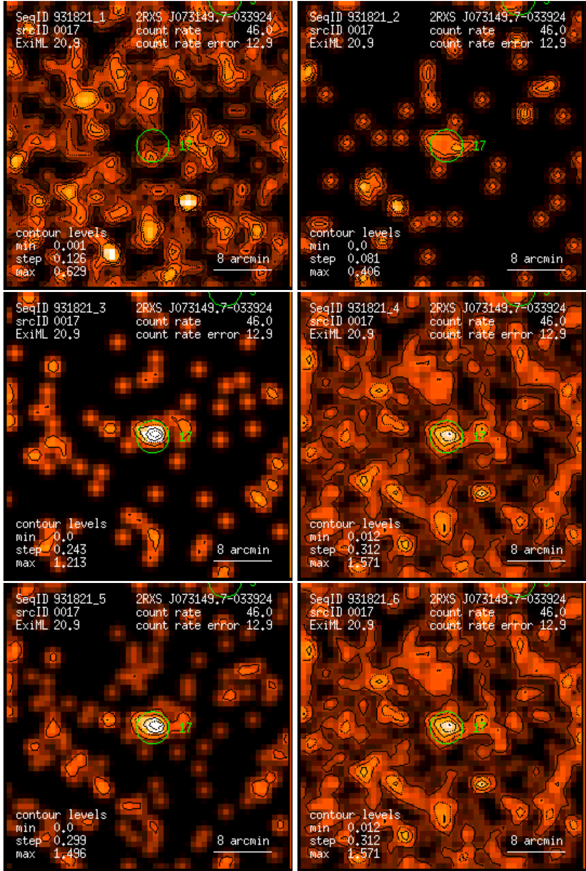
Figure 17: RASS 931821: detection 0017: band rate images, Gaussian filter: (1) PSPC channels 11 – 41, (2) 52 – 90, (3) 91 – 201, (4) 11 – 235, (5) 52 – 201, (6) 11 – 201. Broad band rates in counts/ks. Band rate contour levels in counts/ks/arcmin 2 .
