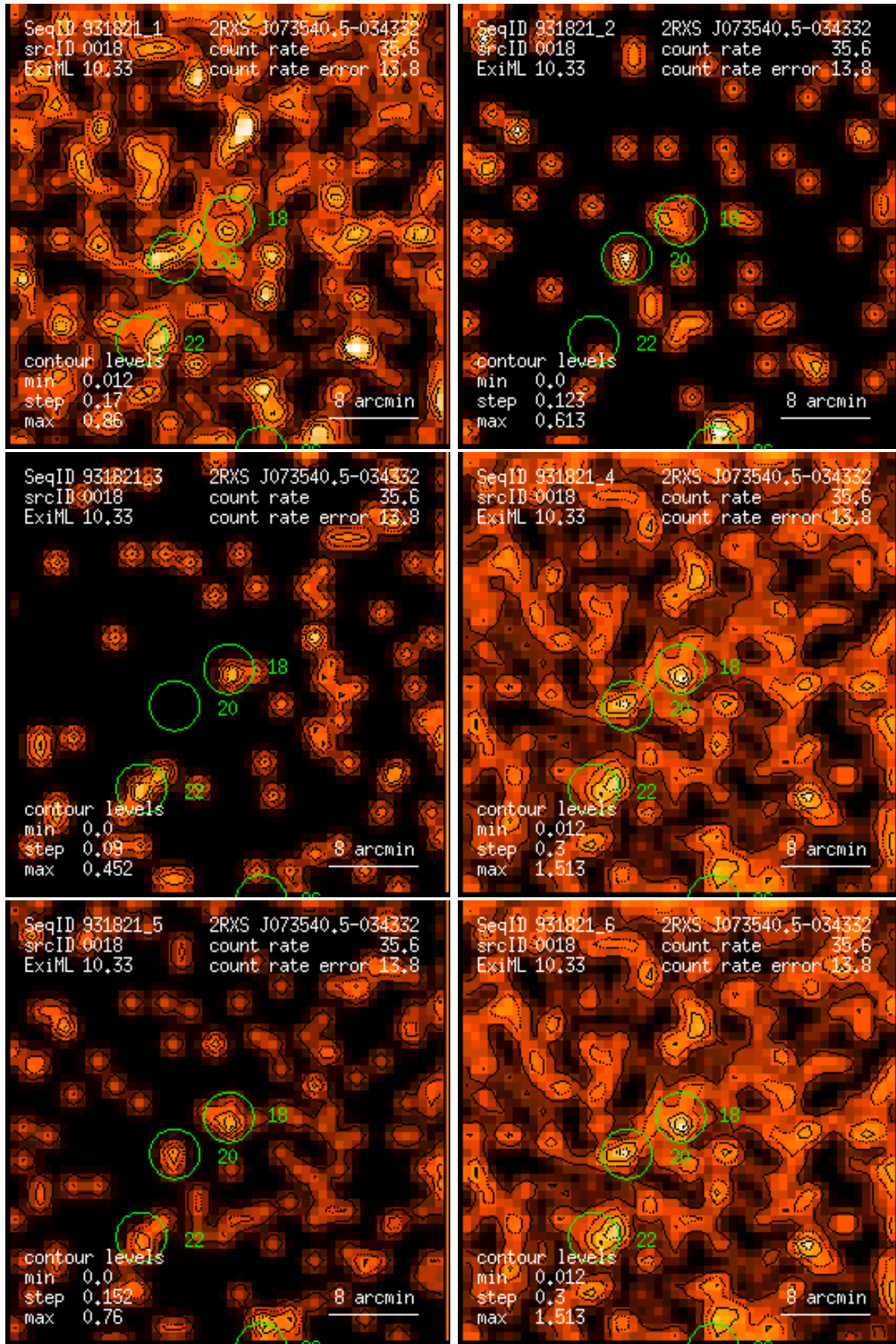
Figure 18: RASS 931821: detection 0018: band rate images, Gaussian filter: (1) PSPC channels 11 – 41, (2) 52 – 90, (3) 91 – 201, (4) 11 – 235, (5) 52 – 201, (6) 11 – 201. Broad band rates in counts/ks. Band rate contour levels in counts/ks/arcmin 2 .
