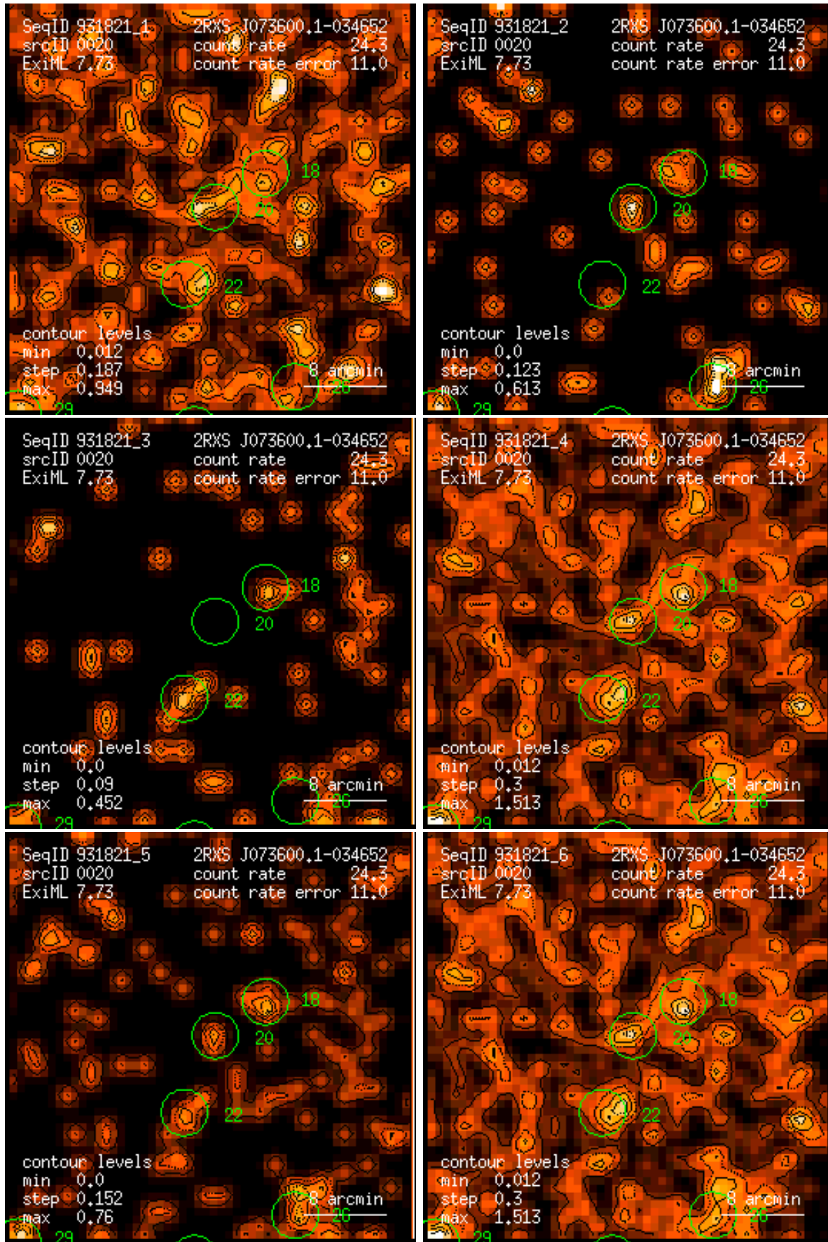
Figure 20: RASS 931821: detection 0020: band rate images, Gaussian filter: (1) PSPC channels 11 – 41, (2) 52 – 90, (3) 91 – 201, (4) 11 – 235, (5) 52 – 201, (6) 11 – 201. Broad band rates in counts/ks. Band rate contour levels in counts/ks/arcmin 2 .
