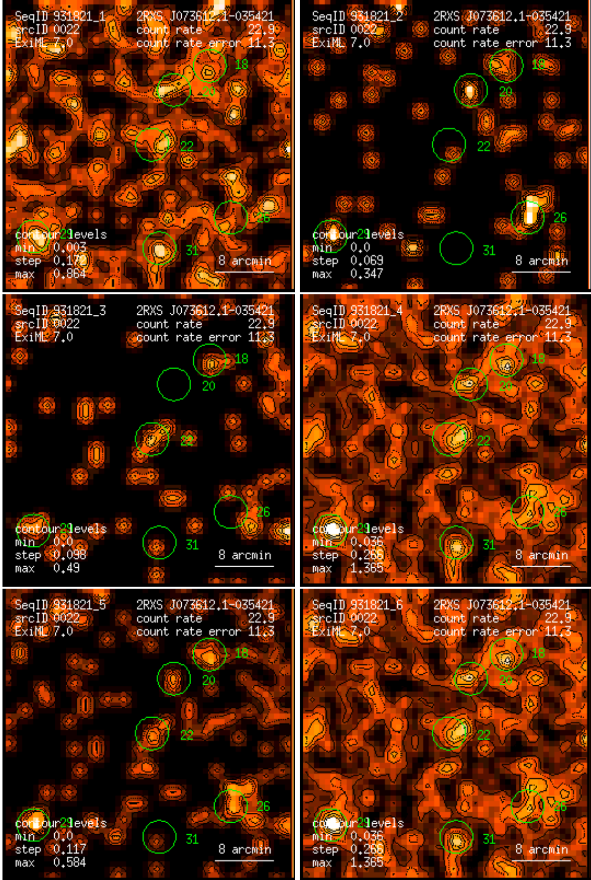
Figure 22: RASS 931821: detection 0022: band rate images, Gaussian filter: (1) PSPC channels 11 – 41, (2) 52 – 90, (3) 91 – 201, (4) 11 – 235, (5) 52 – 201, (6) 11 – 201. Broad band rates in counts/ks. Band rate contour levels in counts/ks/arcmin 2 .
