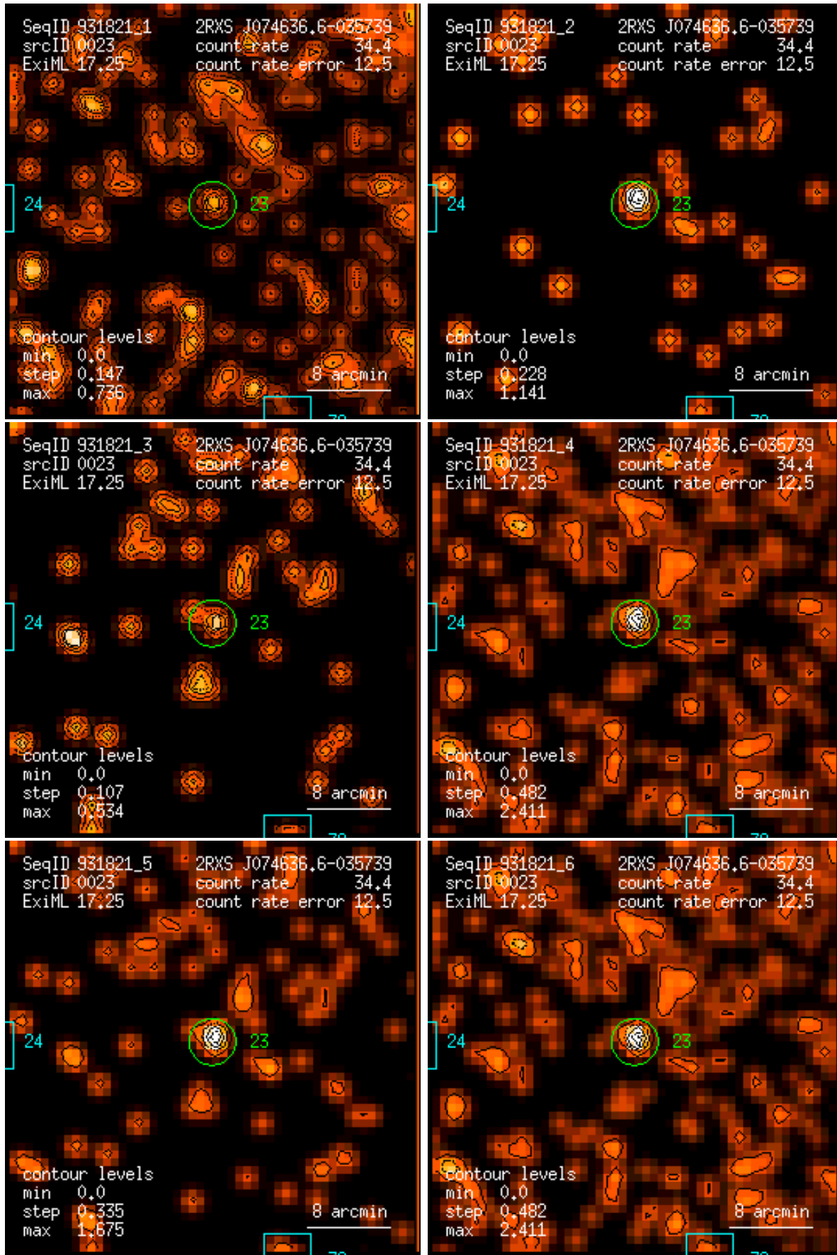
Figure 23: RASS 931821: detection 0023: band rate images, Gaussian filter: (1) PSPC channels 11 – 41, (2) 52 – 90, (3) 91 – 201, (4) 11 – 235, (5) 52 – 201, (6) 11 – 201. Broad band rates in counts/ks. Band rate contour levels in counts/ks/arcmin 2 .
