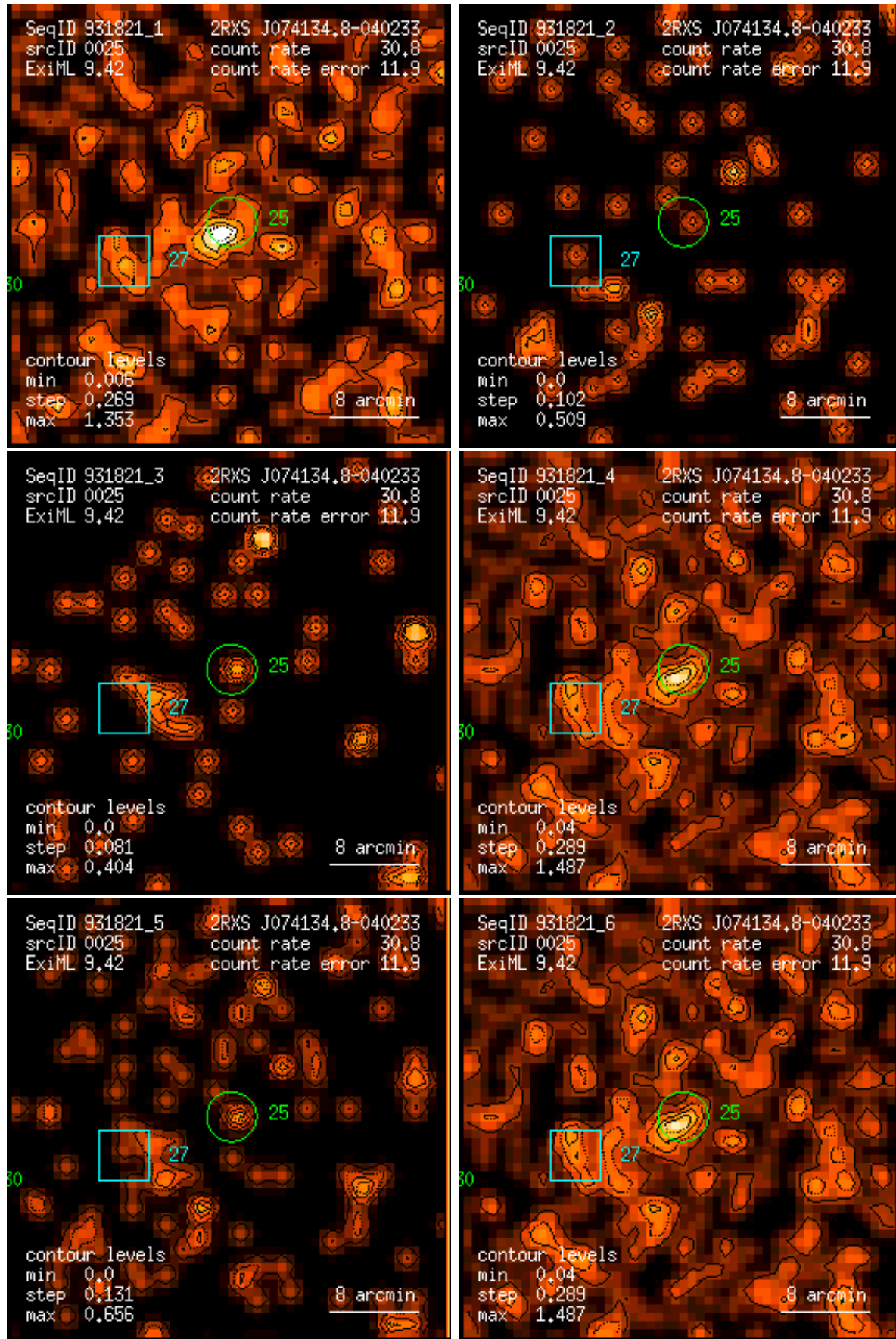
Figure 25: RASS 931821: detection 0025: band rate images, Gaussian filter: (1) PSPC channels 11 – 41, (2) 52 – 90, (3) 91 – 201, (4) 11 – 235, (5) 52 – 201, (6) 11 – 201. Broad band rates in counts/ks. Band rate contour levels in counts/ks/arcmin 2 .
