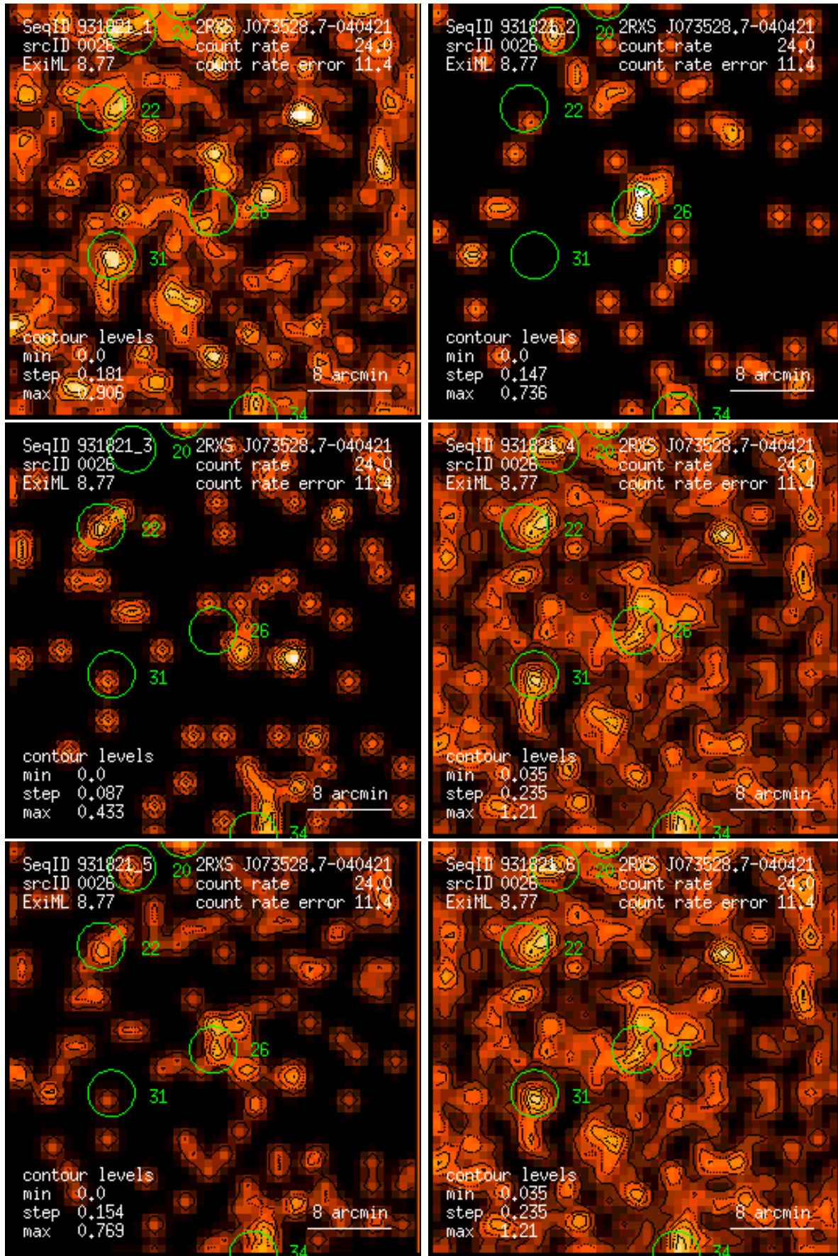
Figure 26: RASS 931821: detection 0026: band rate images, Gaussian filter: (1) PSPC channels 11 – 41, (2) 52 – 90, (3) 91 – 201, (4) 11 – 235, (5) 52 – 201, (6) 11 – 201. Broad band rates in counts/ks. Band rate contour levels in counts/ks/arcmin 2 .
