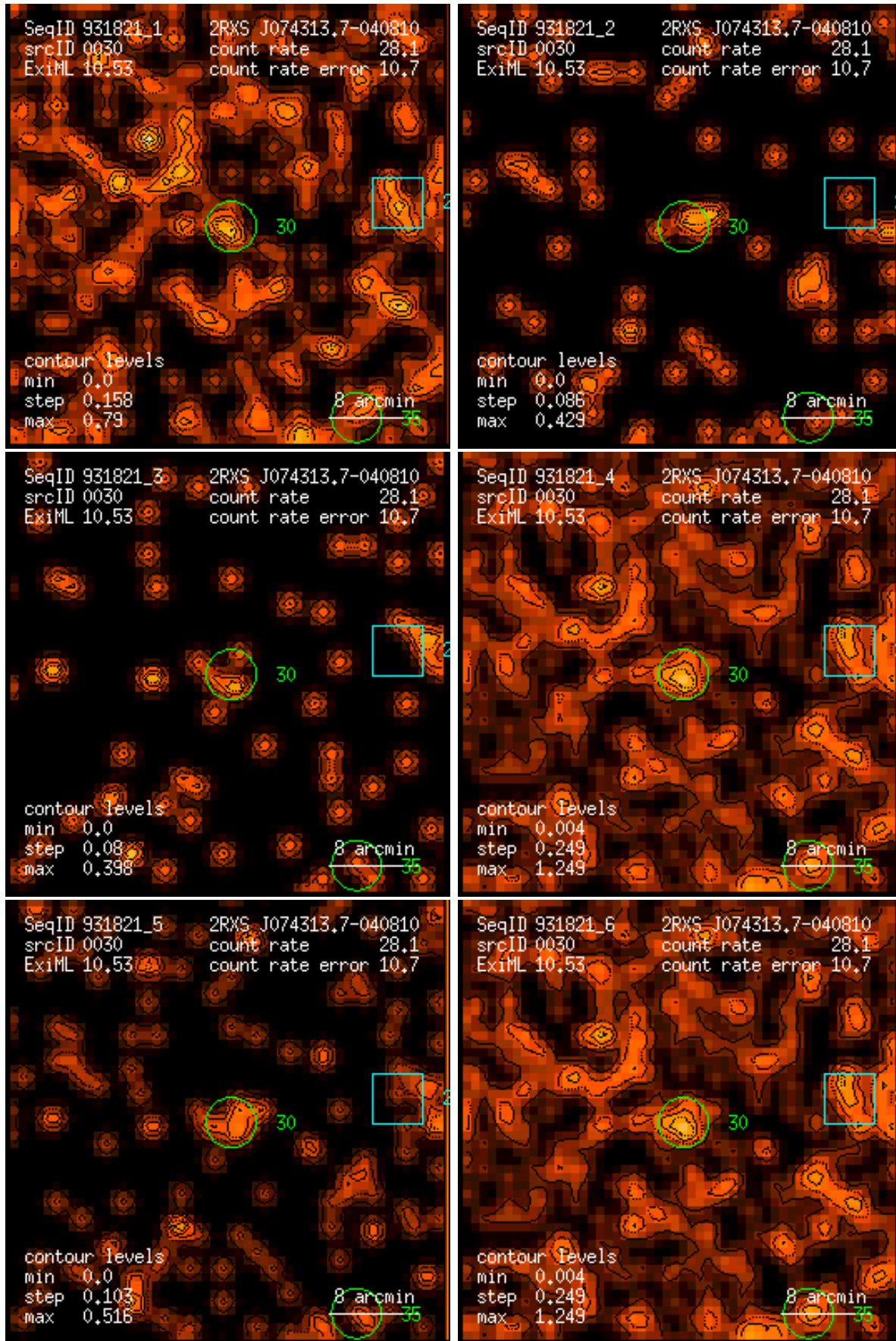
Figure 30: RASS 931821: detection 0030: band rate images, Gaussian filter: (1) PSPC channels 11 – 41, (2) 52 – 90, (3) 91 – 201, (4) 11 – 235, (5) 52 – 201, (6) 11 – 201. Broad band rates in counts/ks. Band rate contour levels in counts/ks/arcmin 2 .
