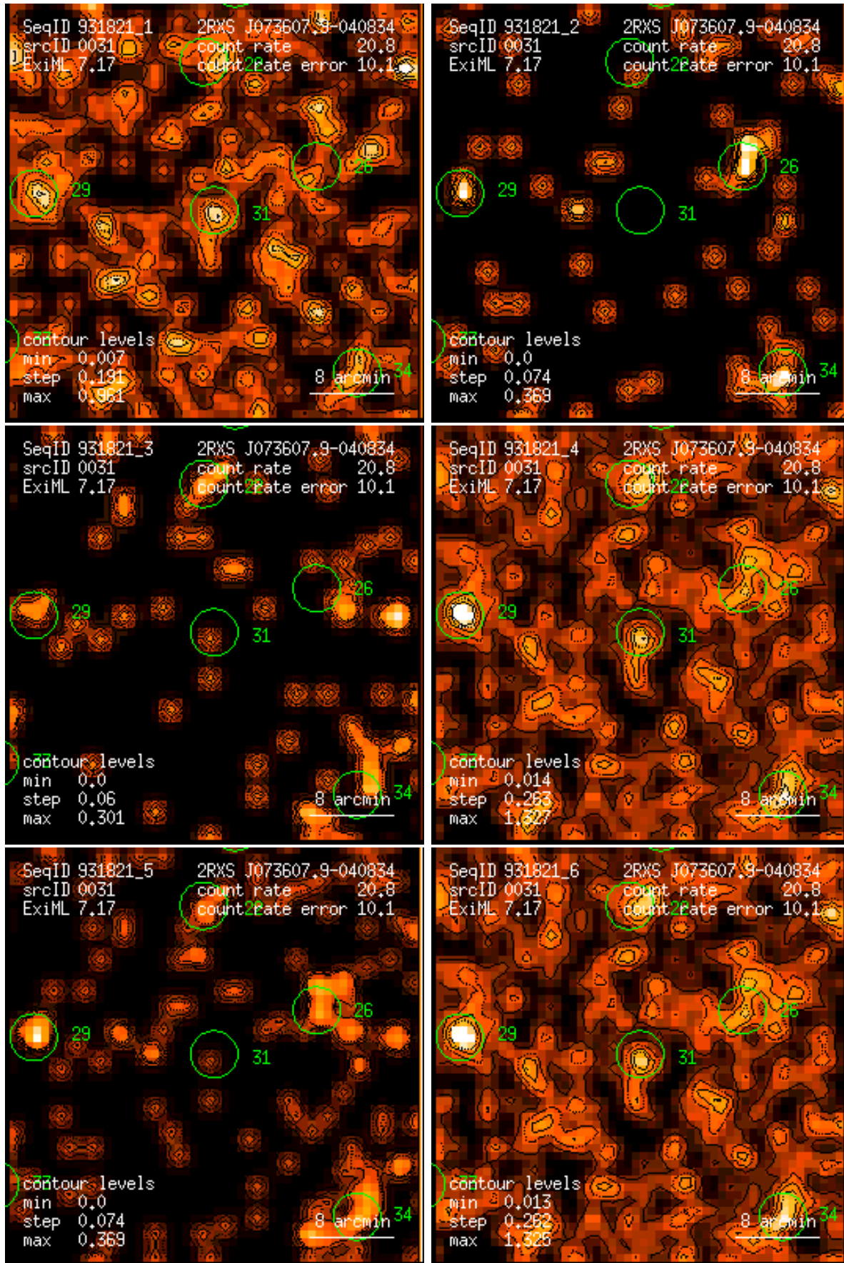
Figure 31: RASS 931821: detection 0031: band rate images, Gaussian filter: (1) PSPC channels 11 – 41, (2) 52 – 90, (3) 91 – 201, (4) 11 – 235, (5) 52 – 201, (6) 11 – 201. Broad band rates in counts/ks. Band rate contour levels in counts/ks/arcmin 2 .
