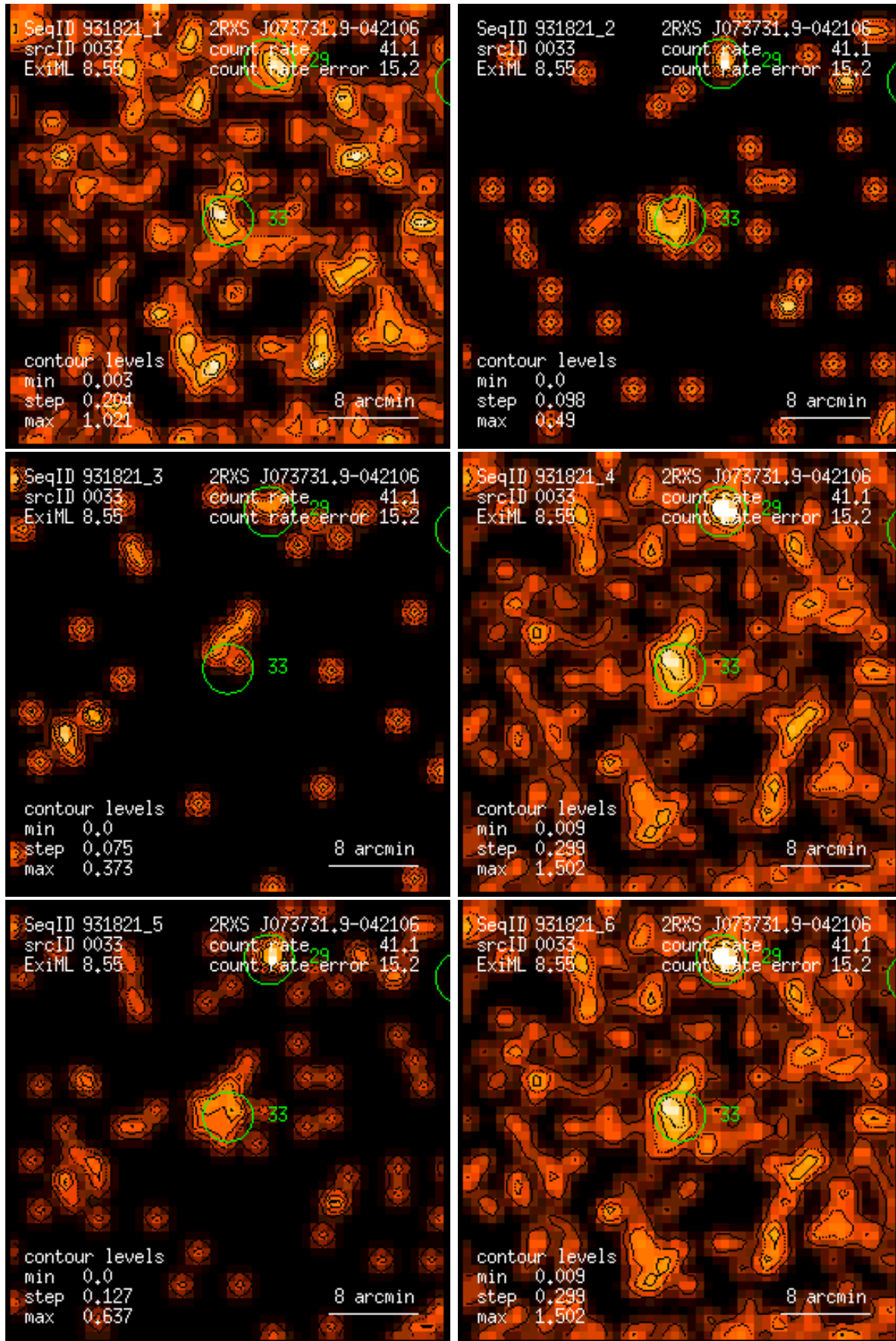
Figure 33: RASS 931821: detection 0033: band rate images, Gaussian filter: (1) PSPC channels 11 – 41, (2) 52 – 90, (3) 91 – 201, (4) 11 – 235, (5) 52 – 201, (6) 11 – 201. Broad band rates in counts/ks. Band rate contour levels in counts/ks/arcmin 2 .
