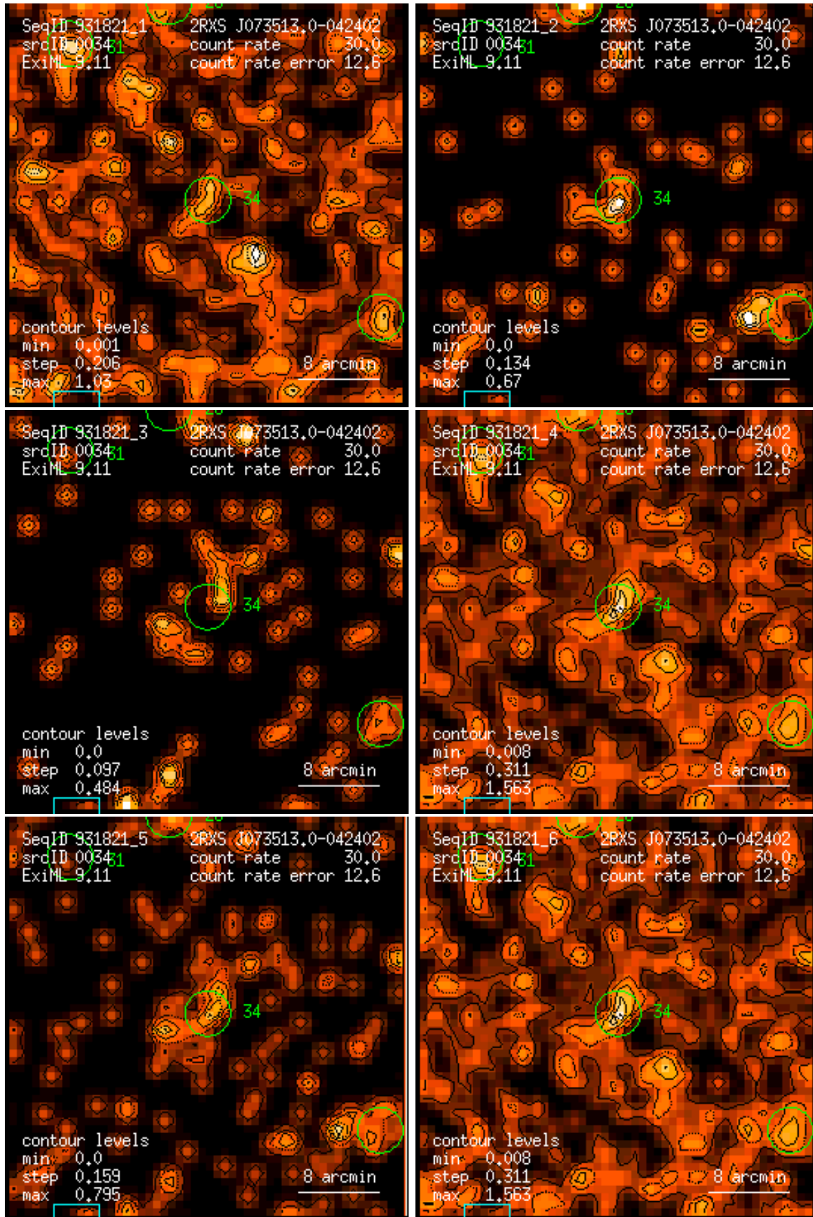
Figure 34: RASS 931821: detection 0034: band rate images, Gaussian filter: (1) PSPC channels 11 – 41, (2) 52 – 90, (3) 91 – 201, (4) 11 – 235, (5) 52 – 201, (6) 11 – 201. Broad band rates in counts/ks. Band rate contour levels in counts/ks/arcmin 2 .
