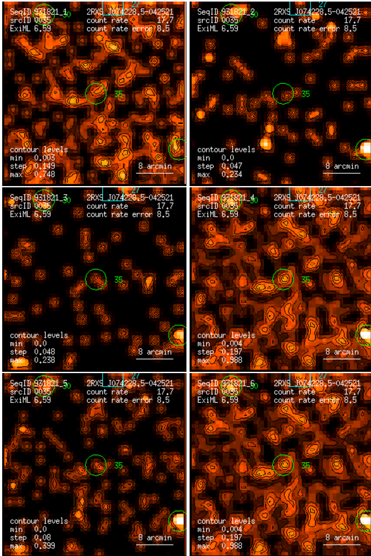
Figure 35: RASS 931821: detection 0035: band rate images, Gaussian filter: (1) PSPC channels 11 – 41, (2) 52 – 90, (3) 91 – 201, (4) 11 – 235, (5) 52 – 201, (6) 11 – 201. Broad band rates in counts/ks. Band rate contour levels in counts/ks/arcmin 2 .
