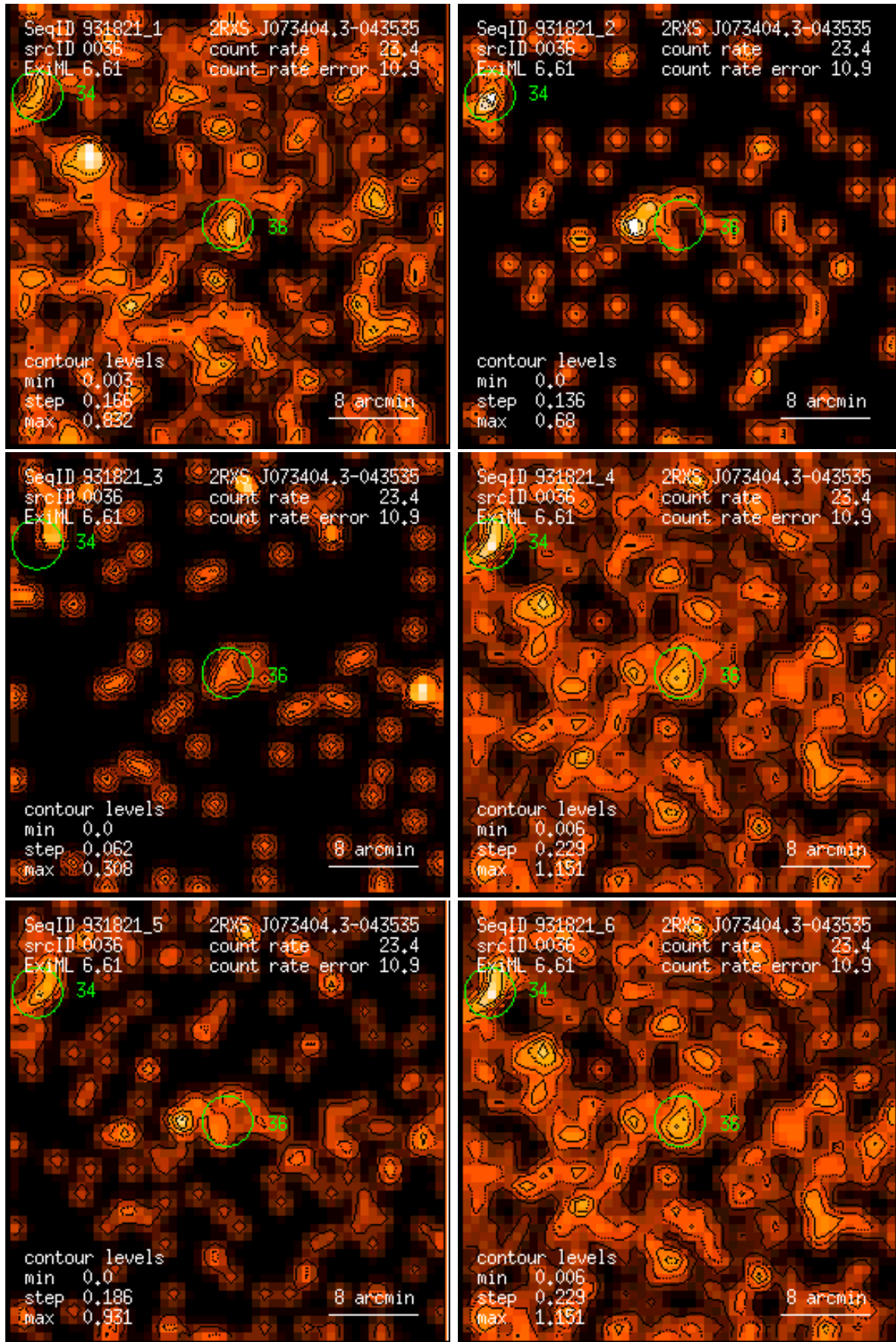
Figure 36: RASS 931821: detection 0036: band rate images, Gaussian filter: (1) PSPC channels 11 – 41, (2) 52 – 90, (3) 91 – 201, (4) 11 – 235, (5) 52 – 201, (6) 11 – 201. Broad band rates in counts/ks. Band rate contour levels in counts/ks/arcmin 2 .
