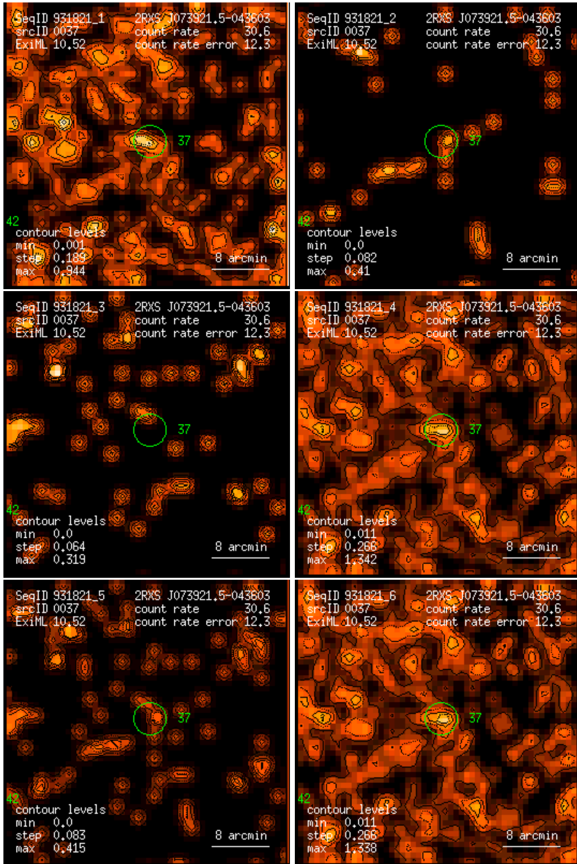
Figure 37: RASS 931821: detection 0037: band rate images, Gaussian filter: (1) PSPC channels 11 – 41, (2) 52 – 90, (3) 91 – 201, (4) 11 – 235, (5) 52 – 201, (6) 11 – 201. Broad band rates in counts/ks. Band rate contour levels in counts/ks/arcmin 2 .
