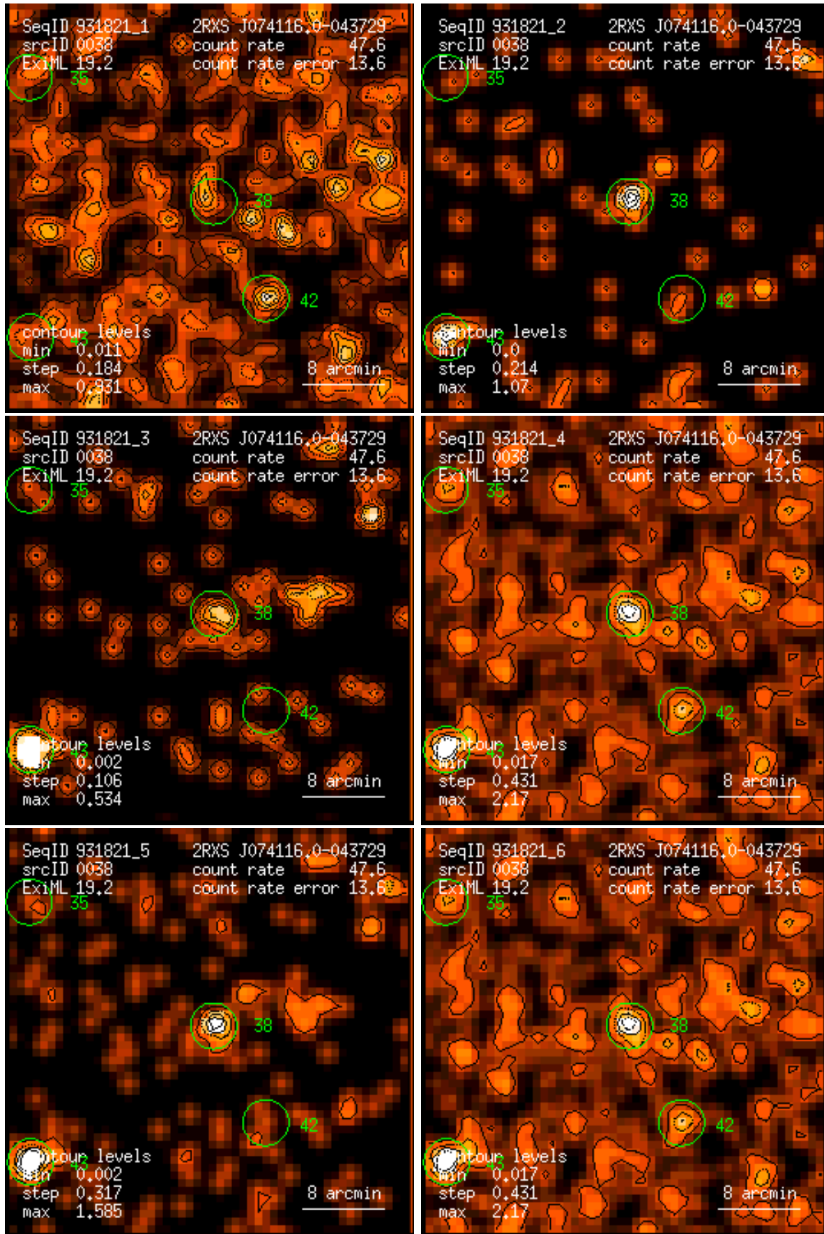
Figure 38: RASS 931821: detection 0038: band rate images, Gaussian filter: (1) PSPC channels 11 – 41, (2) 52 – 90, (3) 91 – 201, (4) 11 – 235, (5) 52 – 201, (6) 11 – 201. Broad band rates in counts/ks. Band rate contour levels in counts/ks/arcmin 2 .
