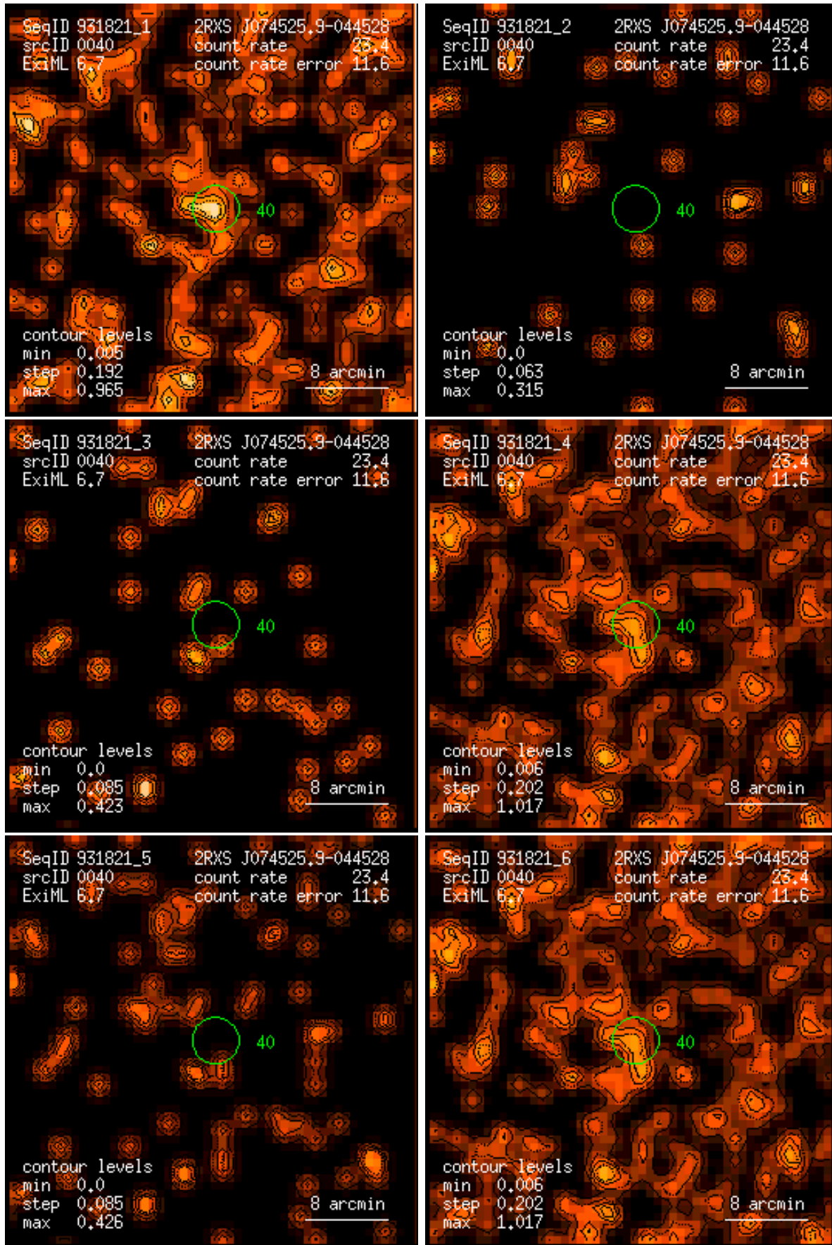
Figure 40: RASS 931821: detection 0040: band rate images, Gaussian filter: (1) PSPC channels 11 – 41, (2) 52 – 90, (3) 91 – 201, (4) 11 – 235, (5) 52 – 201, (6) 11 – 201. Broad band rates in counts/ks. Band rate contour levels in counts/ks/arcmin 2 .
