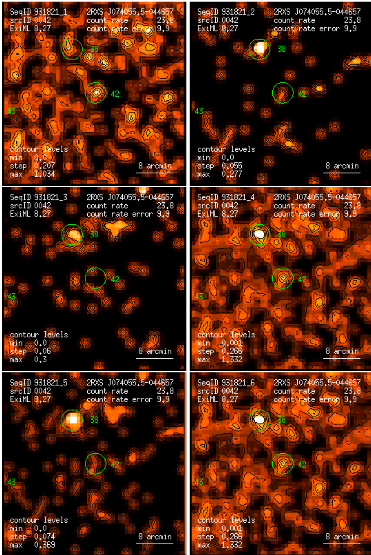
Figure 42: RASS 931821: detection 0042: band rate images, Gaussian filter: (1) PSPC channels 11 – 41, (2) 52 – 90, (3) 91 – 201, (4) 11 – 235, (5) 52 – 201, (6) 11 – 201. Broad band rates in counts/ks. Band rate contour levels in counts/ks/arcmin 2 .
