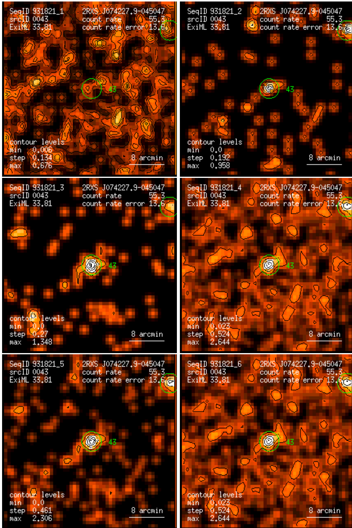
Figure 43: RASS 931821: detection 0043: band rate images, Gaussian filter: (1) PSPC channels 11 – 41, (2) 52 – 90, (3) 91 – 201, (4) 11 – 235, (5) 52 – 201, (6) 11 – 201. Broad band rates in counts/ks. Band rate contour levels in counts/ks/arcmin 2 .
