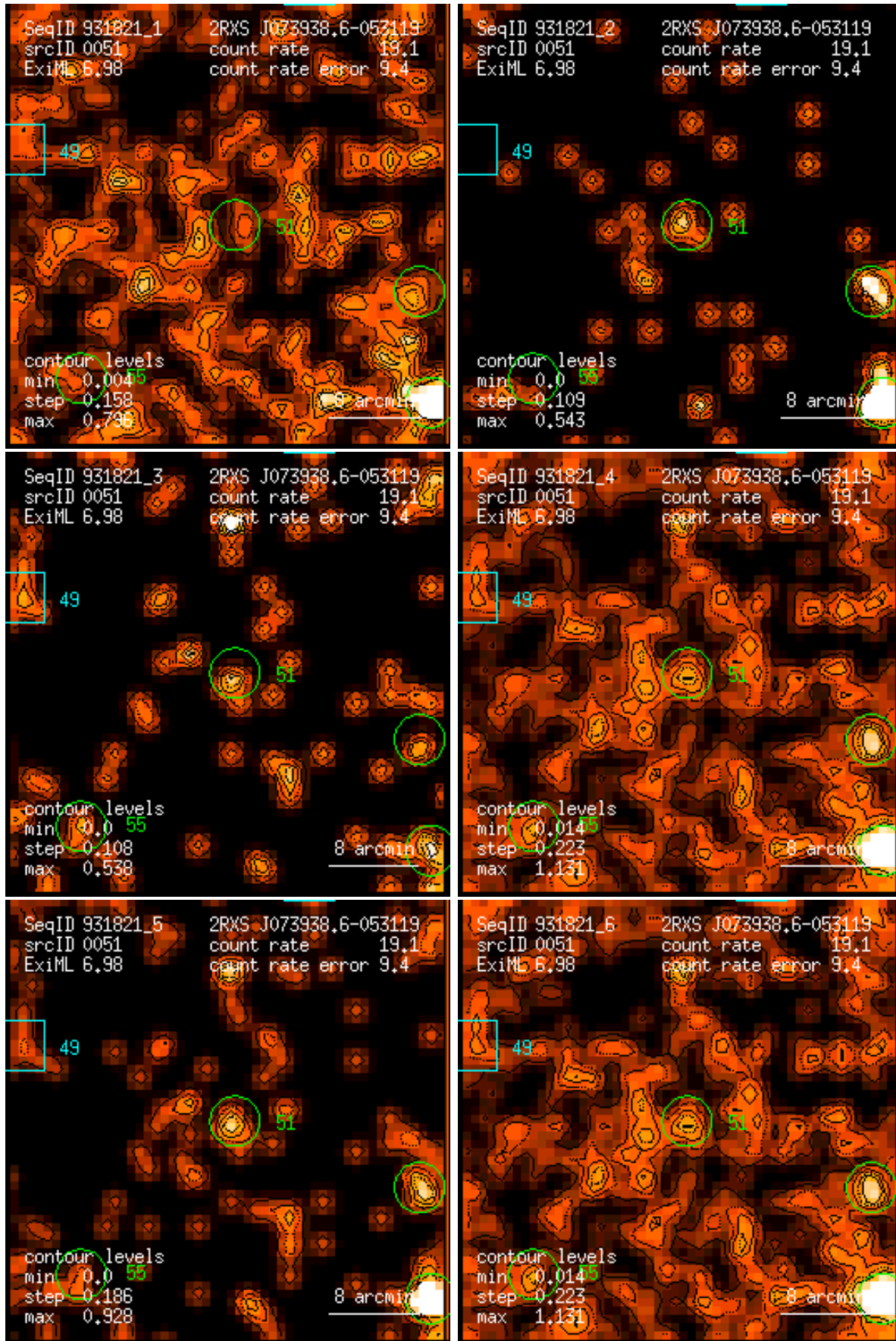
Figure 51: RASS 931821: detection 0051: band rate images, Gaussian filter: (1) PSPC channels 11 – 41, (2) 52 – 90, (3) 91 – 201, (4) 11 – 235, (5) 52 – 201, (6) 11 – 201. Broad band rates in counts/ks. Band rate contour levels in counts/ks/arcmin 2 .
